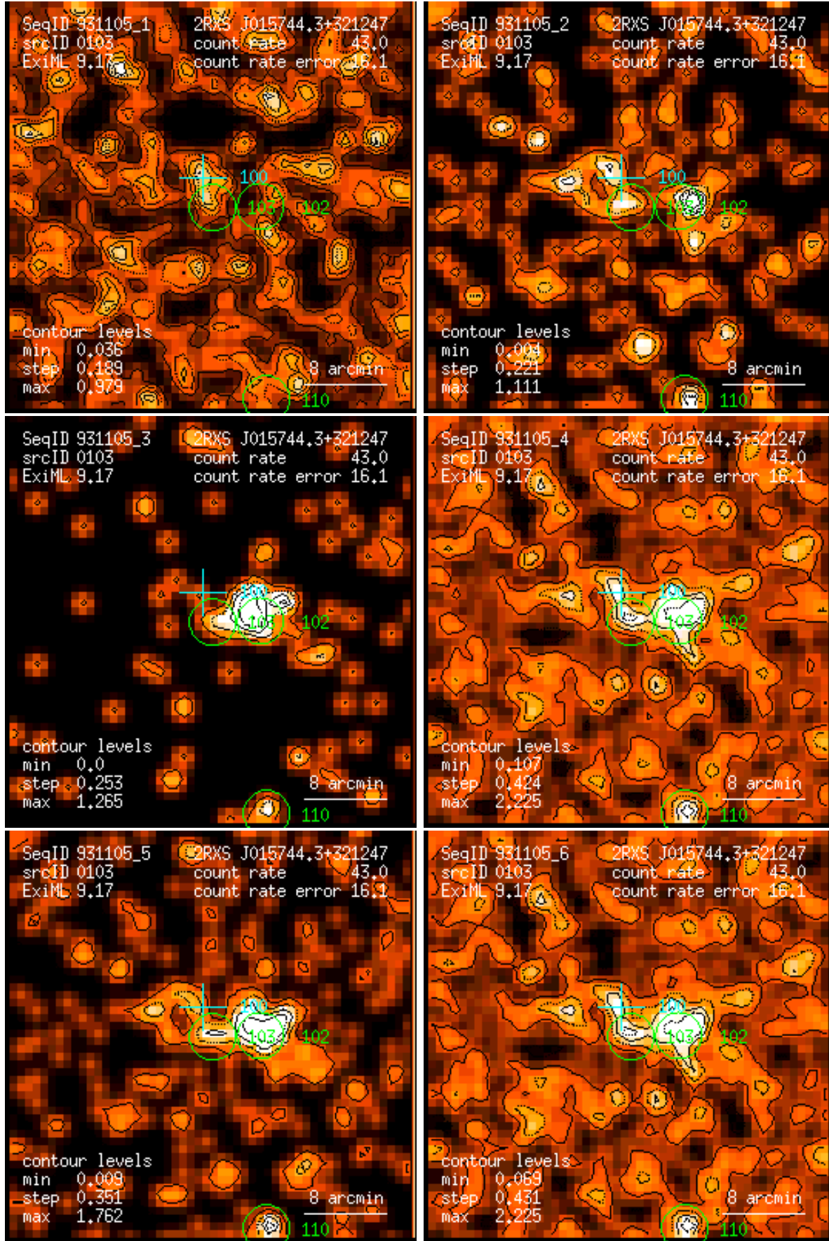
Figure 103: RASS 931105: detection 0103: band rate images, Gaussian filter: (1) PSPC channels 11 – 41, (2) 52 – 90, (3) 91 – 201, (4) 11 – 235, (5) 52 – 201, (6) 11 – 201. Broad band rates in counts/ks. Band rate contour levels in counts/ks/arcmin 2 .
