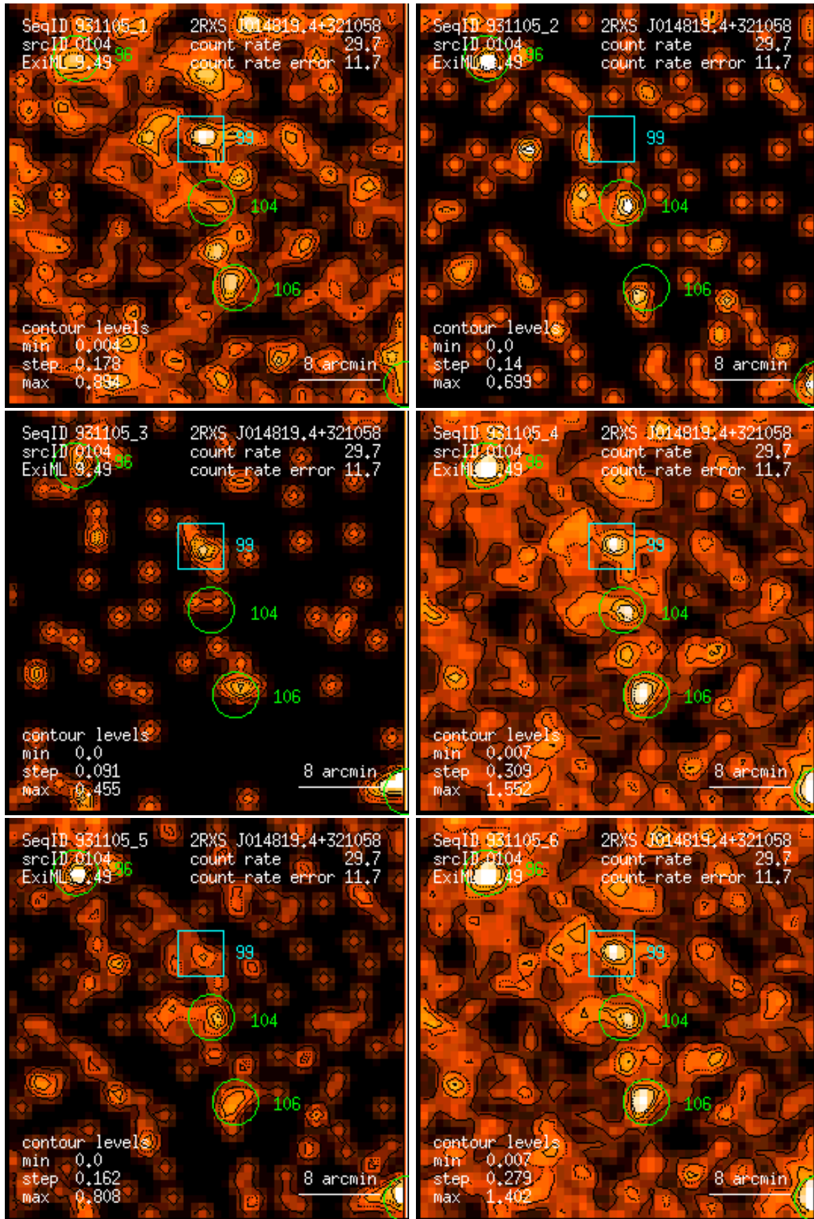
Figure 104: RASS 931105: detection 0104: band rate images, Gaussian filter: (1) PSPC channels 11 – 41, (2) 52 – 90, (3) 91 – 201, (4) 11 – 235, (5) 52 – 201, (6) 11 – 201. Broad band rates in counts/ks. Band rate contour levels in counts/ks/arcmin 2 .
