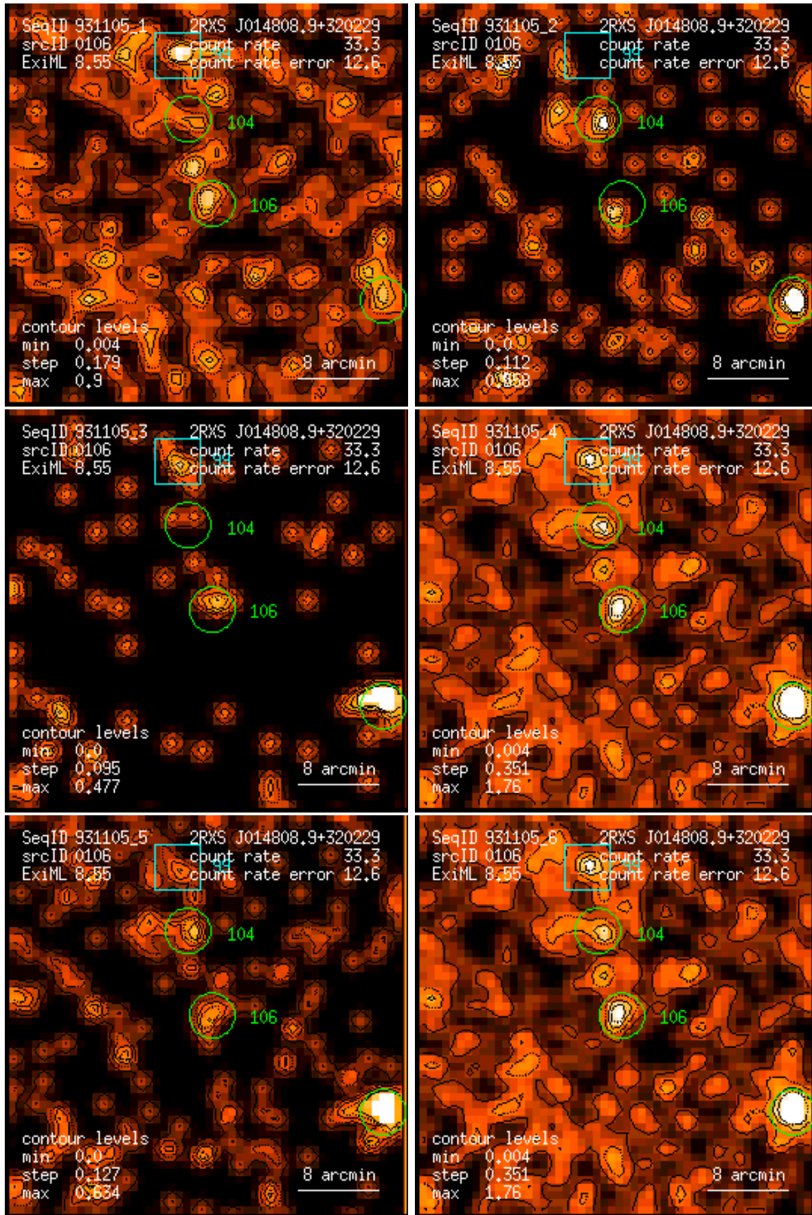
Figure 106: RASS 931105: detection 0106: band rate images, Gaussian filter: (1) PSPC channels 11 – 41, (2) 52 – 90, (3) 91 – 201, (4) 11 – 235, (5) 52 – 201, (6) 11 – 201. Broad band rates in counts/ks. Band rate contour levels in counts/ks/arcmin 2 .
