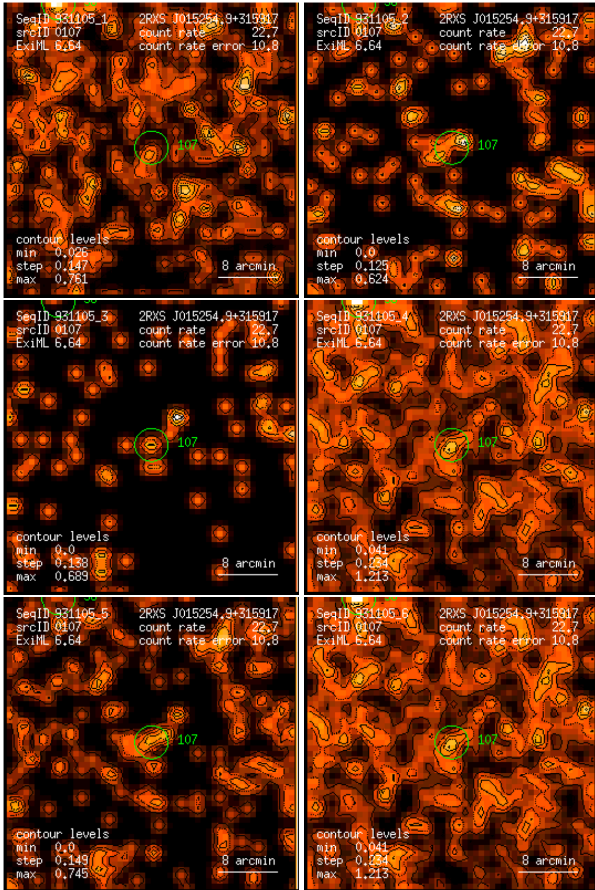
Figure 107: RASS 931105: detection 0107: band rate images, Gaussian filter: (1) PSPC channels 11 – 41, (2) 52 – 90, (3) 91 – 201, (4) 11 – 235, (5) 52 – 201, (6) 11 – 201. Broad band rates in counts/ks. Band rate contour levels in counts/ks/arcmin 2 .
