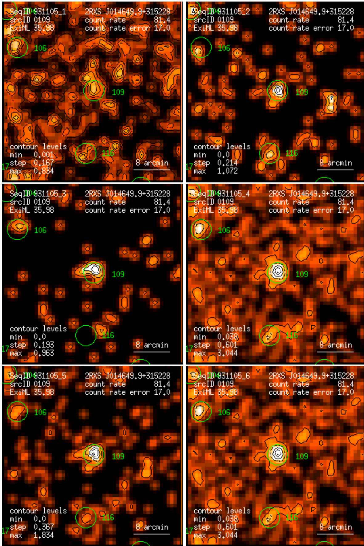
Figure 109: RASS 931105: detection 0109: band rate images, Gaussian filter: (1) PSPC channels 11 – 41, (2) 52 – 90, (3) 91 – 201, (4) 11 – 235, (5) 52 – 201, (6) 11 – 201. Broad band rates in counts/ks. Band rate contour levels in counts/ks/arcmin 2 .
