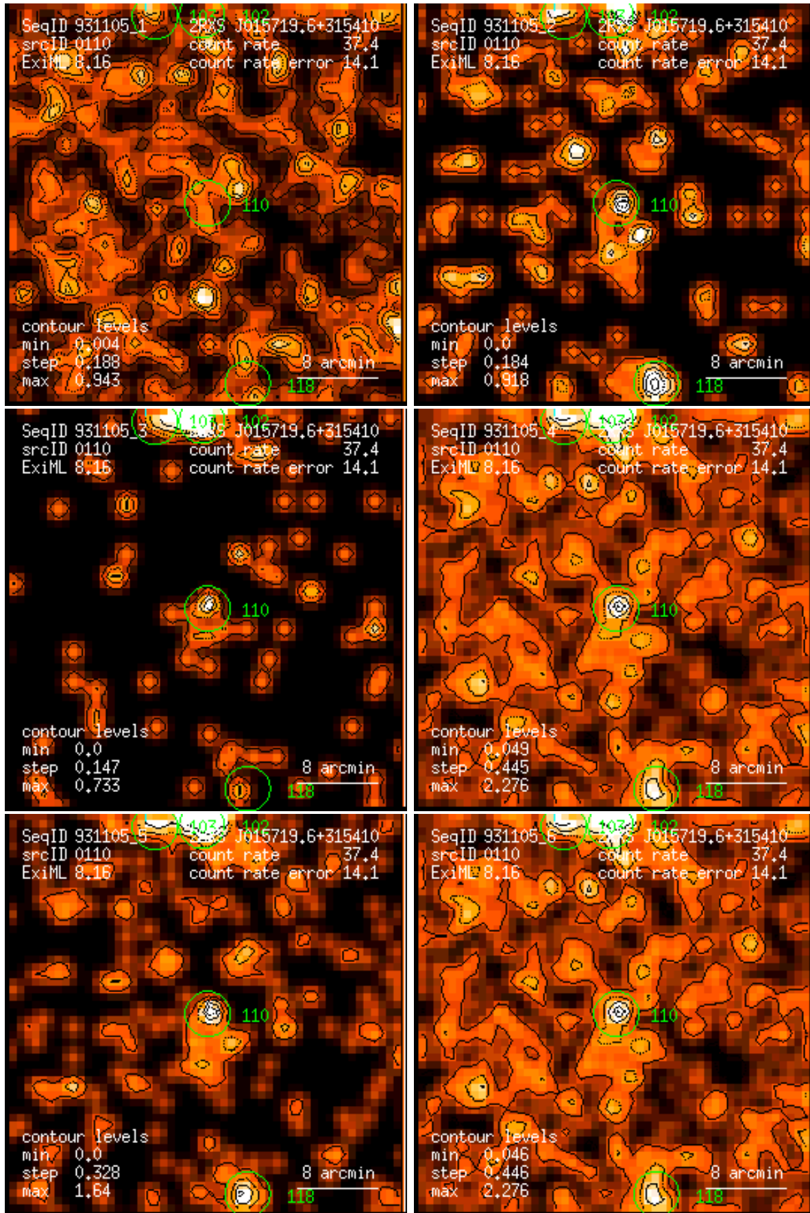
Figure 110: RASS 931105: detection 0110: band rate images, Gaussian filter: (1) PSPC channels 11 – 41, (2) 52 – 90, (3) 91 – 201, (4) 11 – 235, (5) 52 – 201, (6) 11 – 201. Broad band rates in counts/ks. Band rate contour levels in counts/ks/arcmin 2 .
