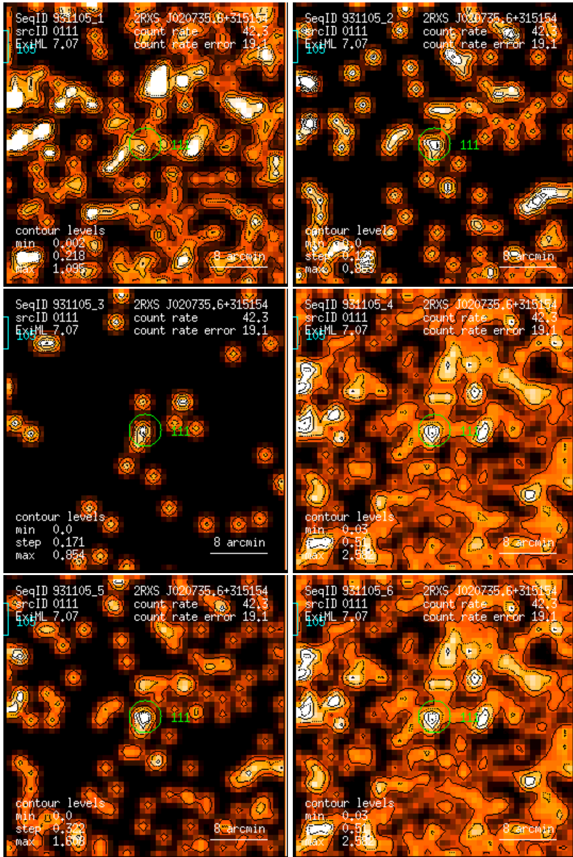
Figure 111: RASS 931105: detection 0111: band rate images, Gaussian filter: (1) PSPC channels 11 – 41, (2) 52 – 90, (3) 91 – 201, (4) 11 – 235, (5) 52 – 201, (6) 11 – 201. Broad band rates in counts/ks. Band rate contour levels in counts/ks/arcmin 2 .
