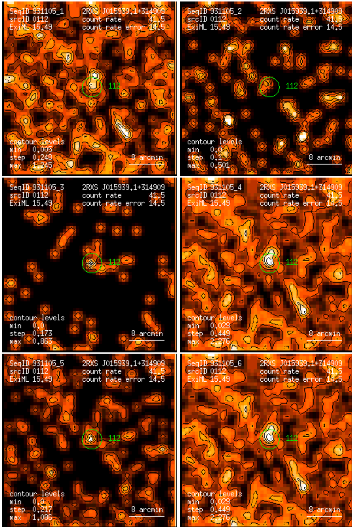
Figure 112: RASS 931105: detection 0112: band rate images, Gaussian filter: (1) PSPC channels 11 – 41, (2) 52 – 90, (3) 91 – 201, (4) 11 – 235, (5) 52 – 201, (6) 11 – 201. Broad band rates in counts/ks. Band rate contour levels in counts/ks/arcmin 2 .
