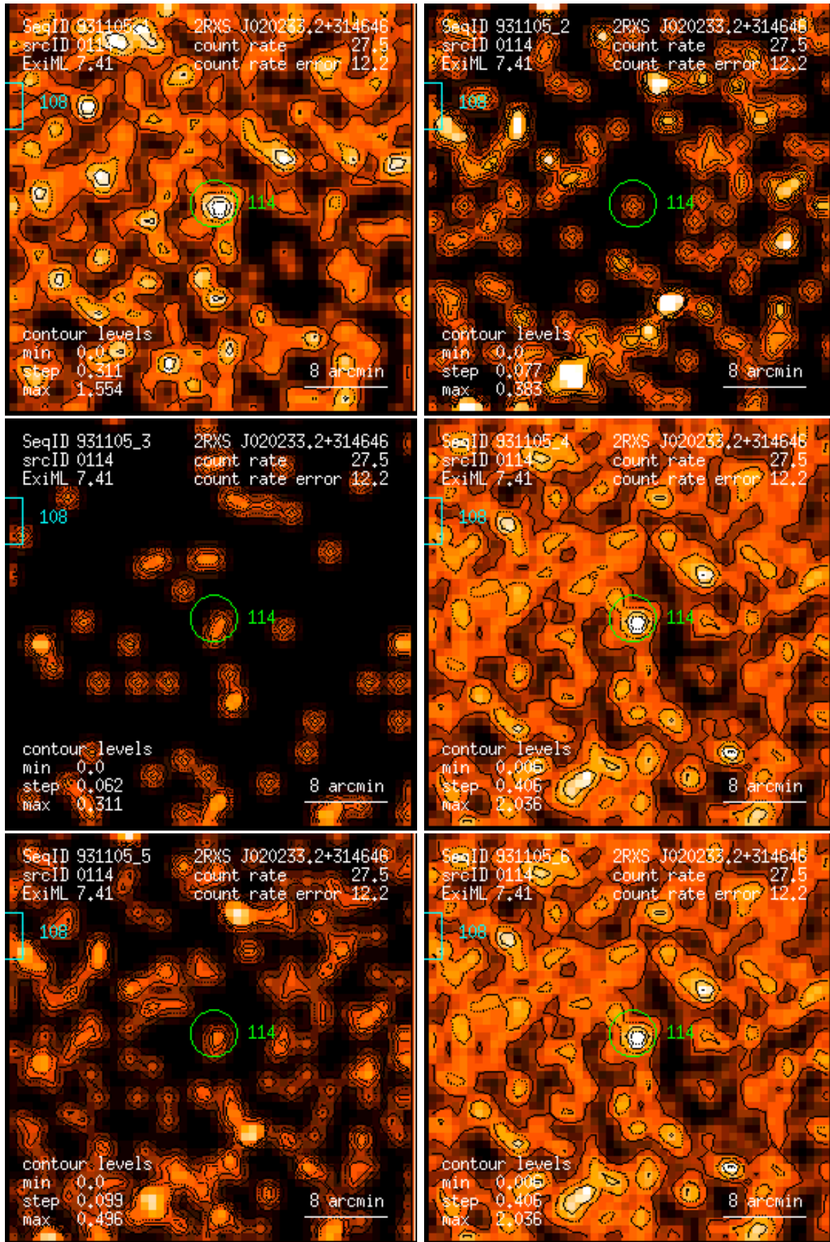
Figure 114: RASS 931105: detection 0114: band rate images, Gaussian filter: (1) PSPC channels 11 – 41, (2) 52 – 90, (3) 91 – 201, (4) 11 – 235, (5) 52 – 201, (6) 11 – 201. Broad band rates in counts/ks. Band rate contour levels in counts/ks/arcmin 2 .
