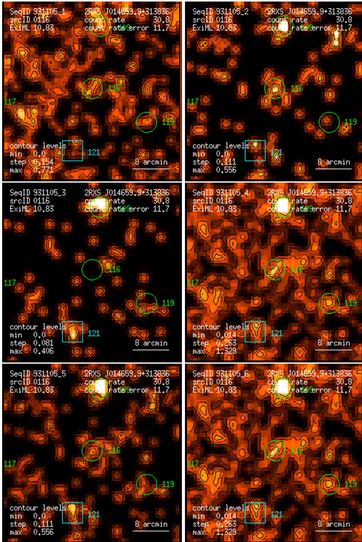
Figure 116: RASS 931105: detection 0116: band rate images, Gaussian filter: (1) PSPC channels 11 – 41, (2) 52 – 90, (3) 91 – 201, (4) 11 – 235, (5) 52 – 201, (6) 11 – 201. Broad band rates in counts/ks. Band rate contour levels in counts/ks/arcmin 2 .
