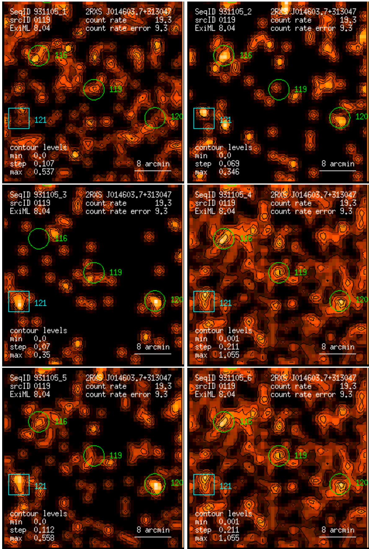
Figure 119: RASS 931105: detection 0119: band rate images, Gaussian filter: (1) PSPC channels 11 – 41, (2) 52 – 90, (3) 91 – 201, (4) 11 – 235, (5) 52 – 201, (6) 11 – 201. Broad band rates in counts/ks. Band rate contour levels in counts/ks/arcmin 2 .
