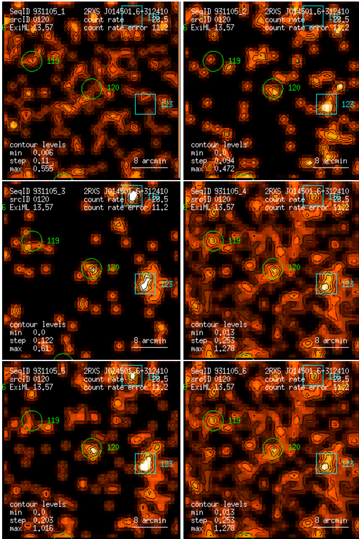
Figure 120: RASS 931105: detection 0120: band rate images, Gaussian filter: (1) PSPC channels 11 – 41, (2) 52 – 90, (3) 91 – 201, (4) 11 – 235, (5) 52 – 201, (6) 11 – 201. Broad band rates in counts/ks. Band rate contour levels in counts/ks/arcmin 2 .
