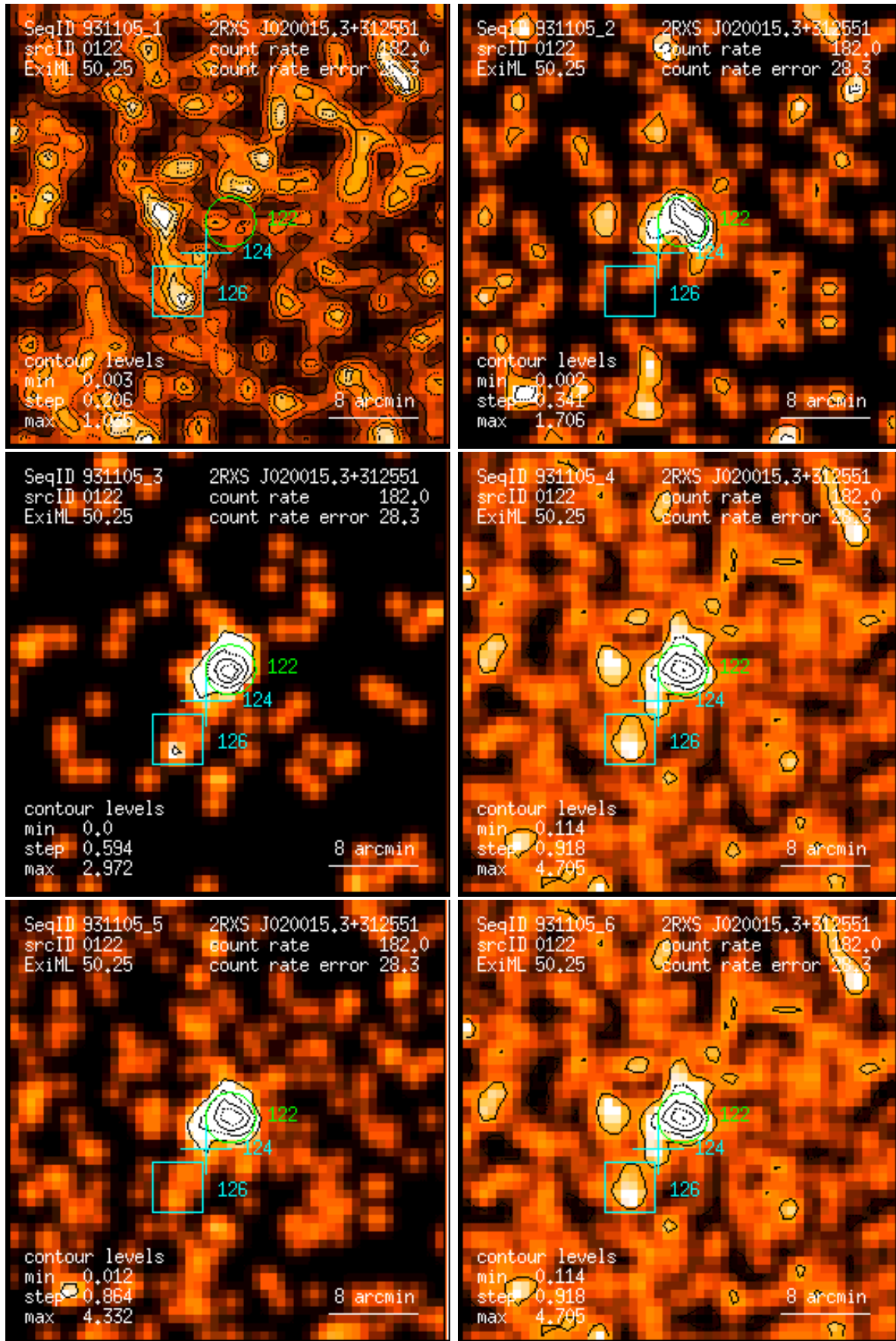
Figure 122: RASS 931105: detection 0122: band rate images, Gaussian filter: (1) PSPC channels 11 – 41, (2) 52 – 90, (3) 91 – 201, (4) 11 – 235, (5) 52 – 201, (6) 11 – 201. Broad band rates in counts/ks. Band rate contour levels in counts/ks/arcmin 2 .
