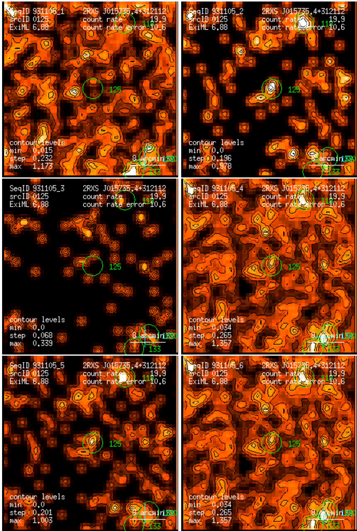
Figure 125: RASS 931105: detection 0125: band rate images, Gaussian filter: (1) PSPC channels 11 – 41, (2) 52 – 90, (3) 91 – 201, (4) 11 – 235, (5) 52 – 201, (6) 11 – 201. Broad band rates in counts/ks. Band rate contour levels in counts/ks/arcmin 2 .
