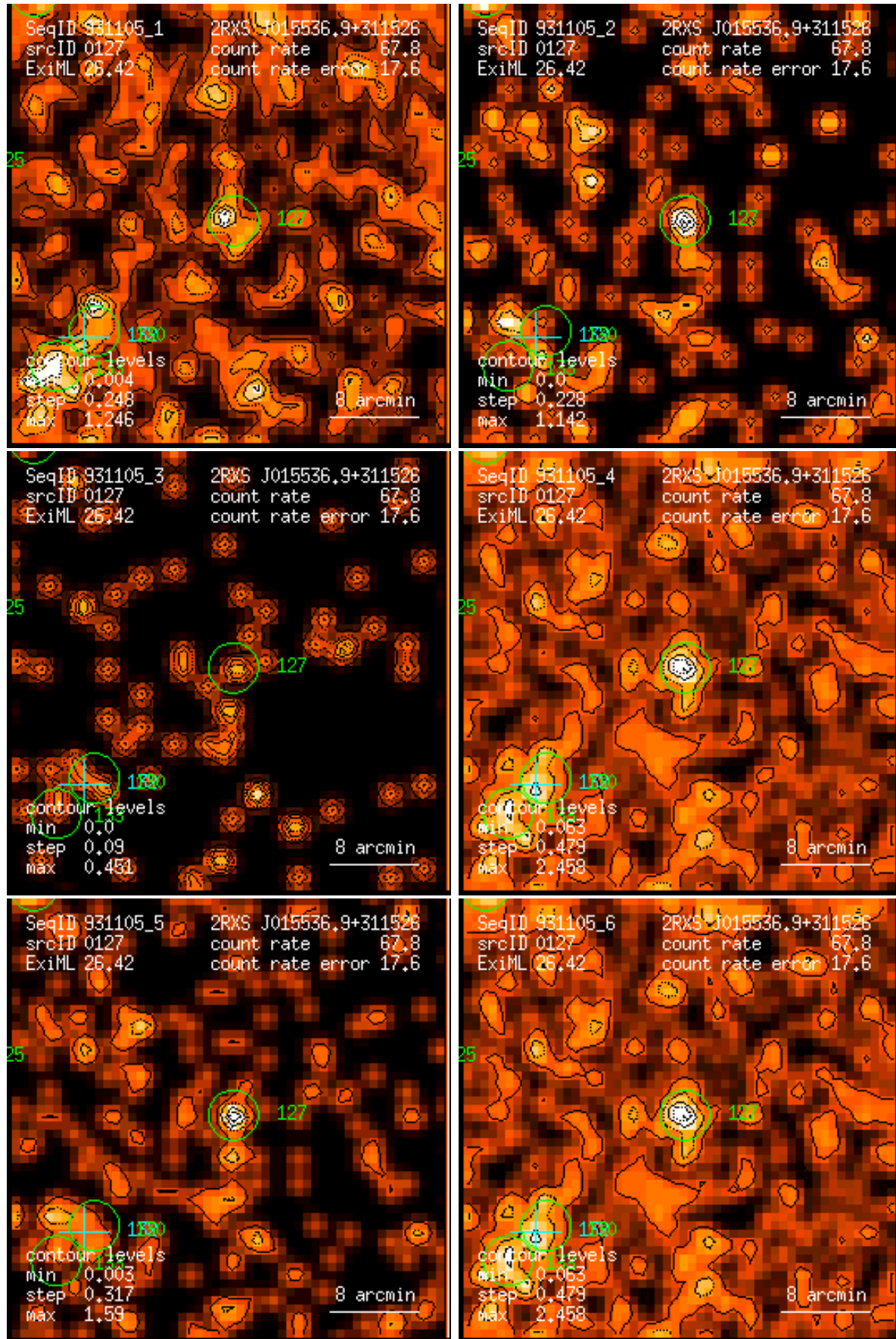
Figure 127: RASS 931105: detection 0127: band rate images, Gaussian filter: (1) PSPC channels 11 – 41, (2) 52 – 90, (3) 91 – 201, (4) 11 – 235, (5) 52 – 201, (6) 11 – 201. Broad band rates in counts/ks. Band rate contour levels in counts/ks/arcmin 2 .
