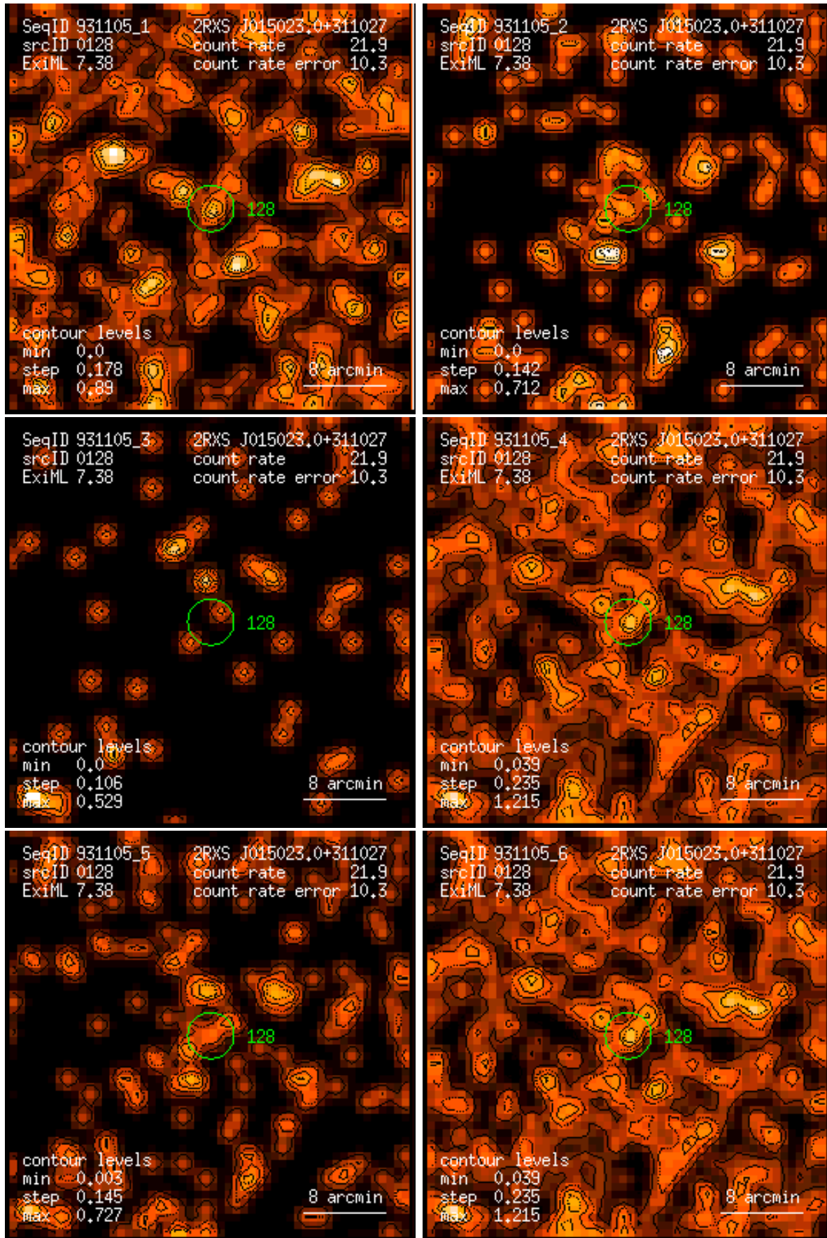
Figure 128: RASS 931105: detection 0128: band rate images, Gaussian filter: (1) PSPC channels 11 – 41, (2) 52 – 90, (3) 91 – 201, (4) 11 – 235, (5) 52 – 201, (6) 11 – 201. Broad band rates in counts/ks. Band rate contour levels in counts/ks/arcmin 2 .
