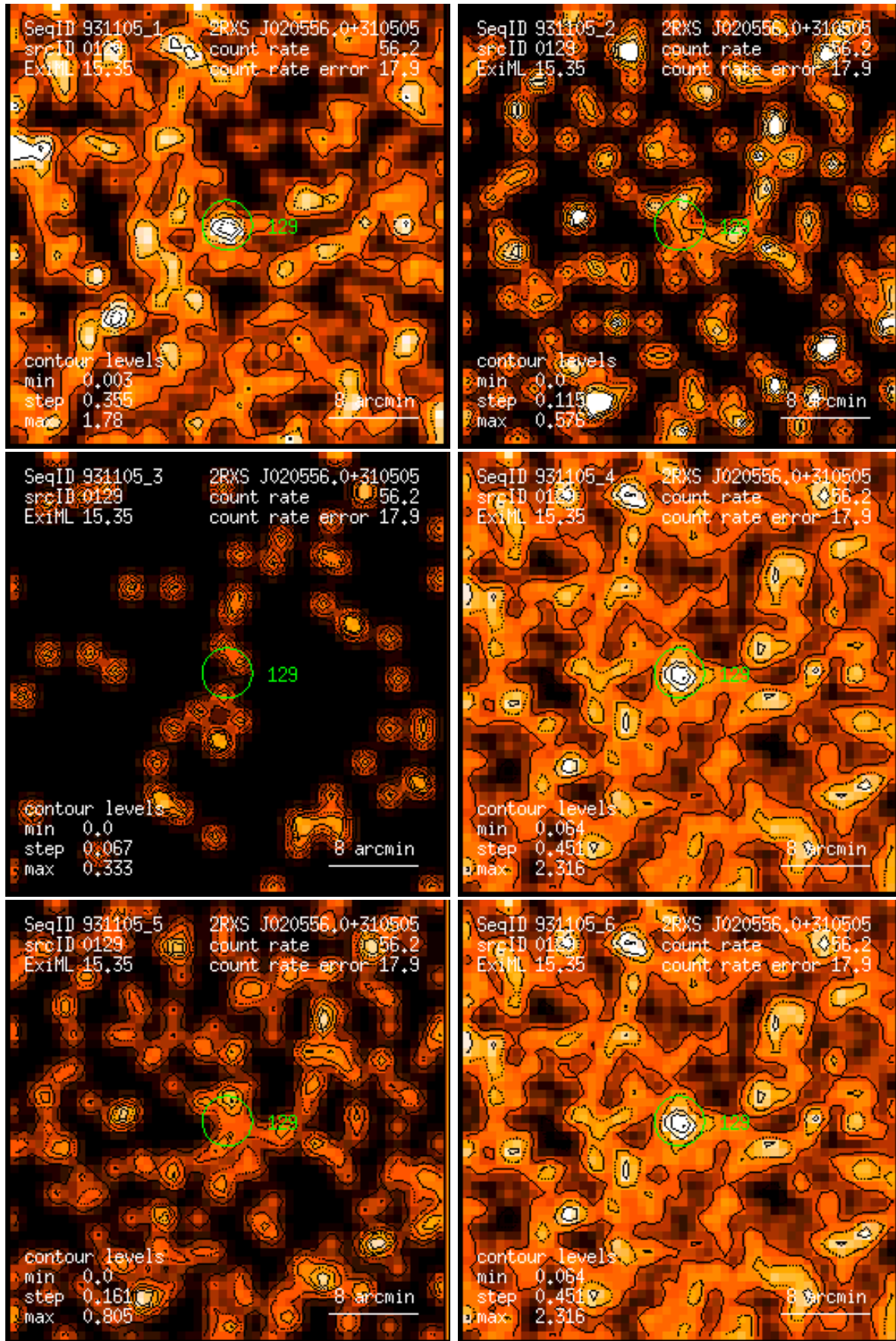
Figure 129: RASS 931105: detection 0129: band rate images, Gaussian filter: (1) PSPC channels 11 – 41, (2) 52 – 90, (3) 91 – 201, (4) 11 – 235, (5) 52 – 201, (6) 11 – 201. Broad band rates in counts/ks. Band rate contour levels in counts/ks/arcmin 2 .
