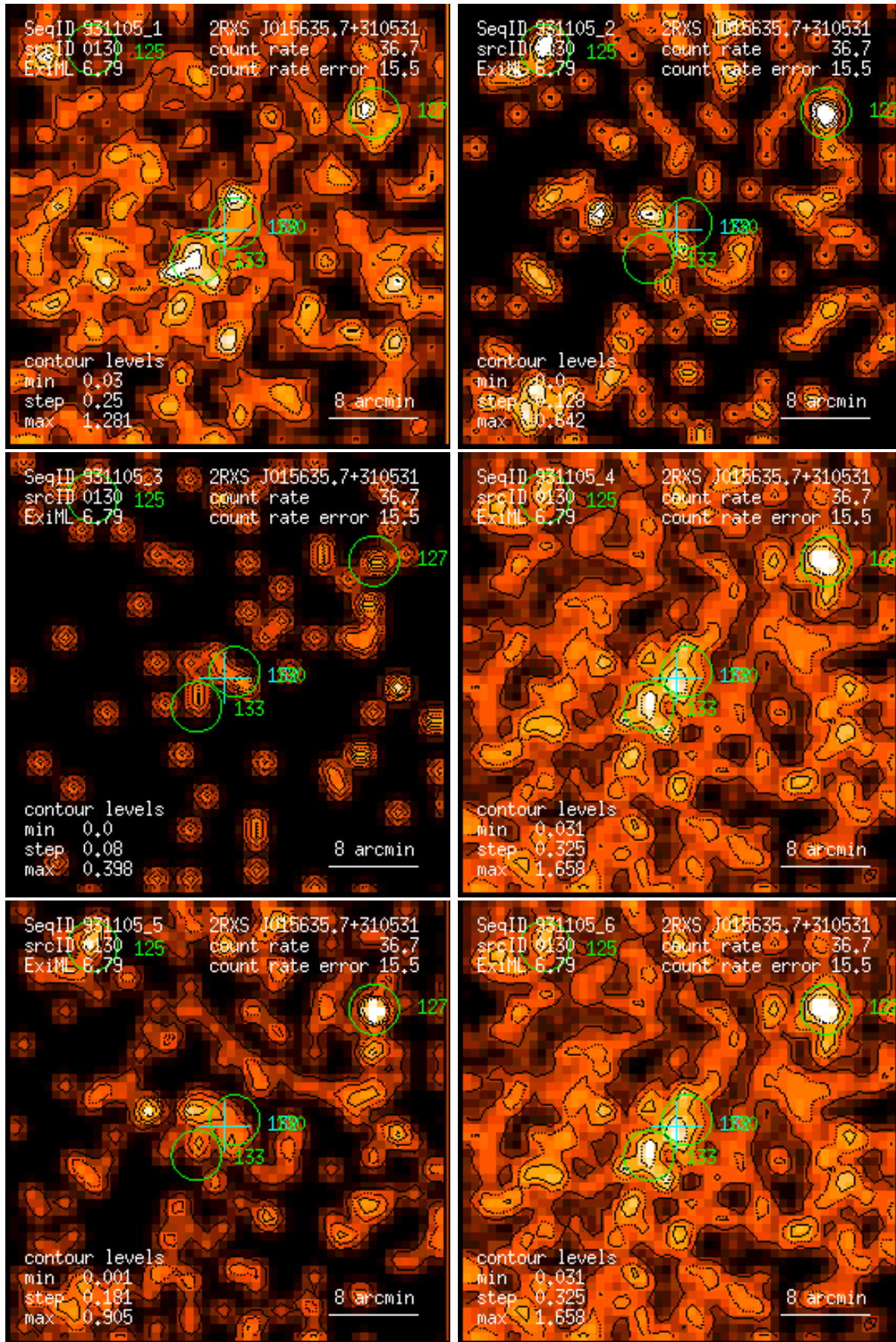
Figure 130: RASS 931105: detection 0130: band rate images, Gaussian filter: (1) PSPC channels 11 – 41, (2) 52 – 90, (3) 91 – 201, (4) 11 – 235, (5) 52 – 201, (6) 11 – 201. Broad band rates in counts/ks. Band rate contour levels in counts/ks/arcmin 2 .
