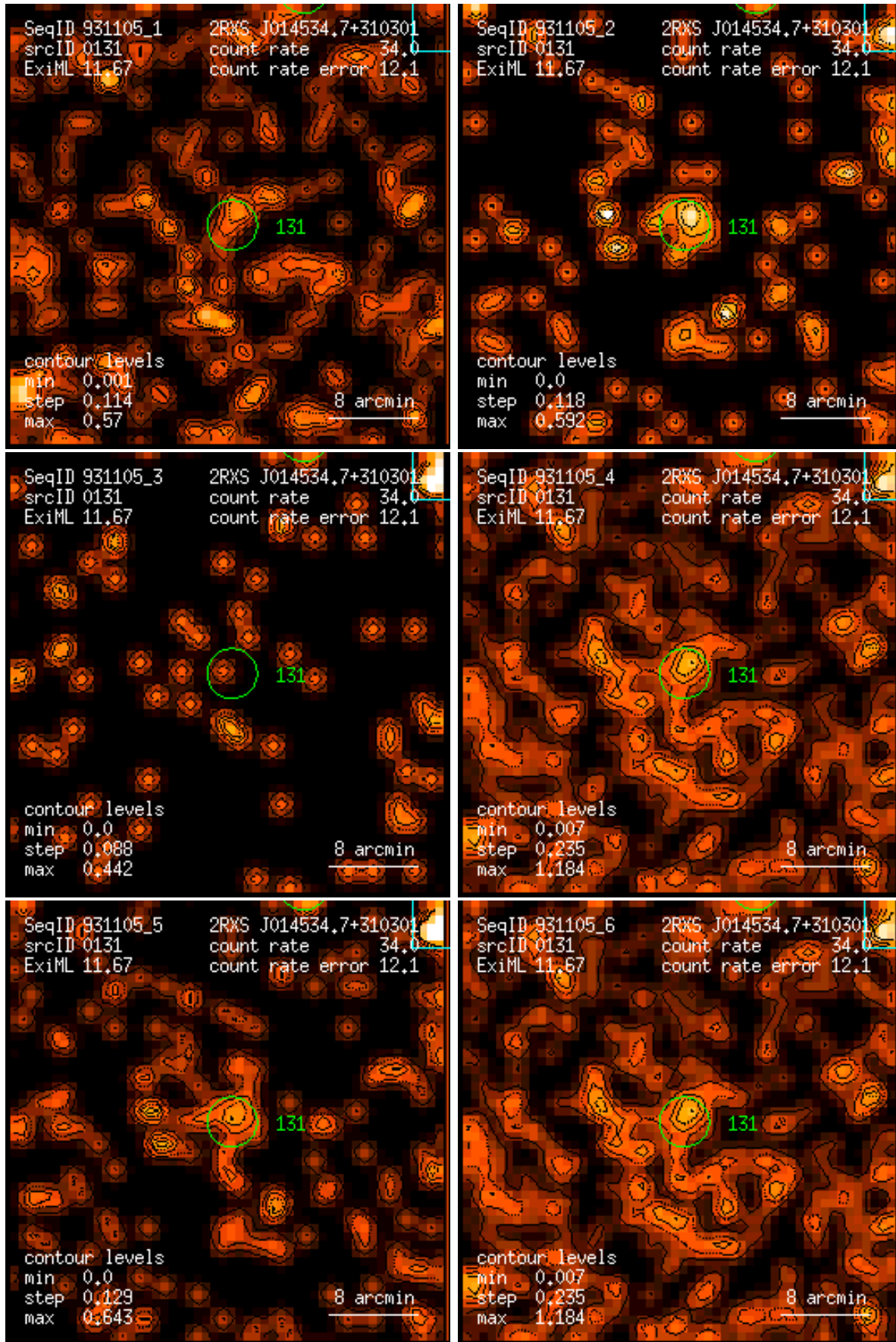
Figure 131: RASS 931105: detection 0131: band rate images, Gaussian filter: (1) PSPC channels 11 – 41, (2) 52 – 90, (3) 91 – 201, (4) 11 – 235, (5) 52 – 201, (6) 11 – 201. Broad band rates in counts/ks. Band rate contour levels in counts/ks/arcmin 2 .
