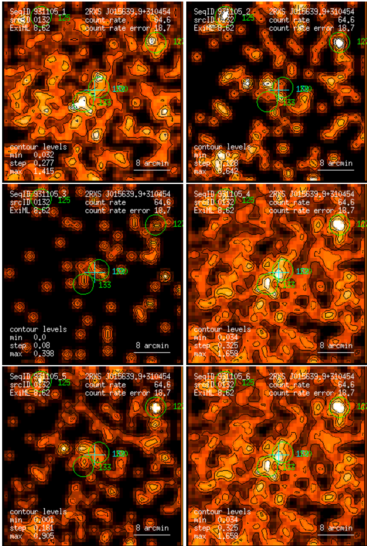
Figure 132: RASS 931105: detection 0132: band rate images, Gaussian filter: (1) PSPC channels 11 – 41, (2) 52 – 90, (3) 91 – 201, (4) 11 – 235, (5) 52 – 201, (6) 11 – 201. Broad band rates in counts/ks. Band rate contour levels in counts/ks/arcmin 2 .
