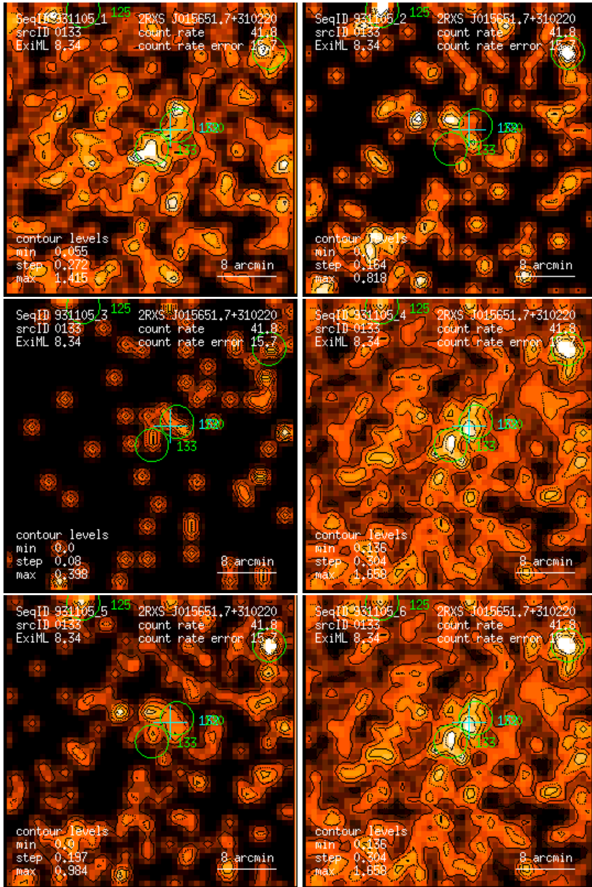
Figure 133: RASS 931105: detection 0133: band rate images, Gaussian filter: (1) PSPC channels 11 – 41, (2) 52 – 90, (3) 91 – 201, (4) 11 – 235, (5) 52 – 201, (6) 11 – 201. Broad band rates in counts/ks. Band rate contour levels in counts/ks/arcmin 2 .
