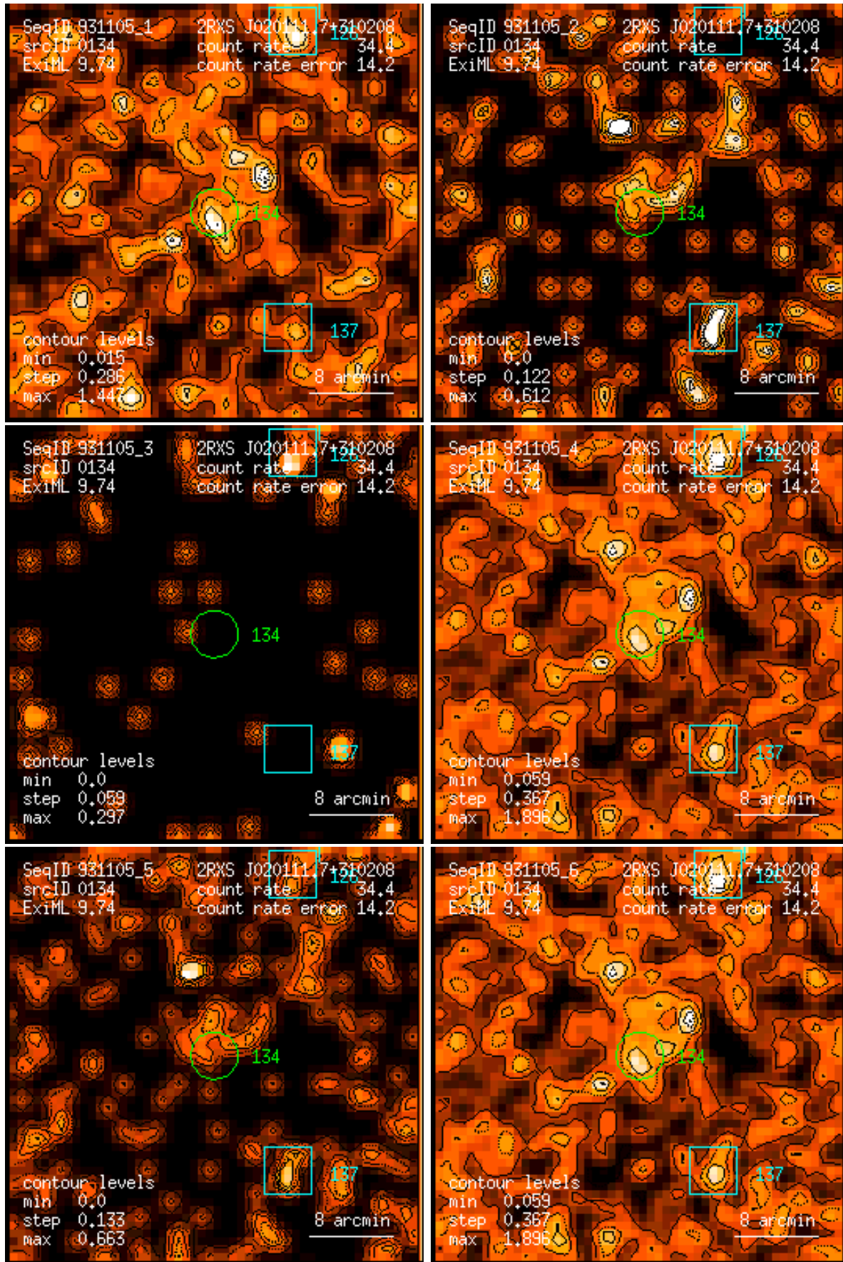
Figure 134: RASS 931105: detection 0134: band rate images, Gaussian filter: (1) PSPC channels 11 – 41, (2) 52 – 90, (3) 91 – 201, (4) 11 – 235, (5) 52 – 201, (6) 11 – 201. Broad band rates in counts/ks. Band rate contour levels in counts/ks/arcmin 2 .
