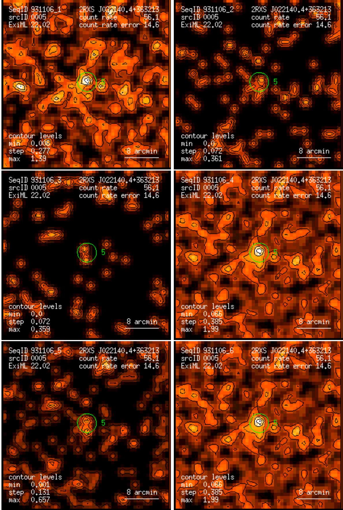
Figure 5: RASS 931106: detection 0005: band rate images, Gaussian filter: (1) PSPC channels 11 – 41, (2) 52 – 90, (3) 91 – 201, (4) 11 – 235, (5) 52 – 201, (6) 11 – 201. Broad band rates in counts/ks. Band rate contour levels in counts/ks/arcmin 2 .
