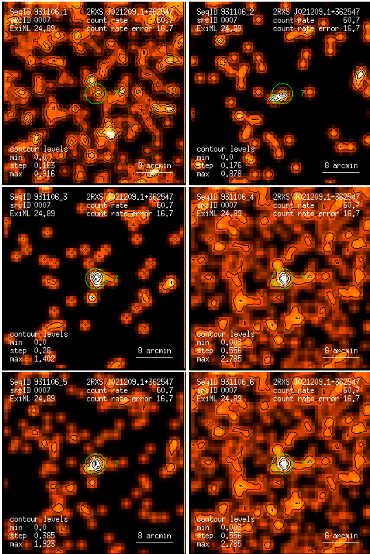
Figure 7: RASS 931106: detection 0007: band rate images, Gaussian filter: (1) PSPC channels 11 – 41, (2) 52 – 90, (3) 91 – 201, (4) 11 – 235, (5) 52 – 201, (6) 11 – 201. Broad band rates in counts/ks. Band rate contour levels in counts/ks/arcmin 2 .
