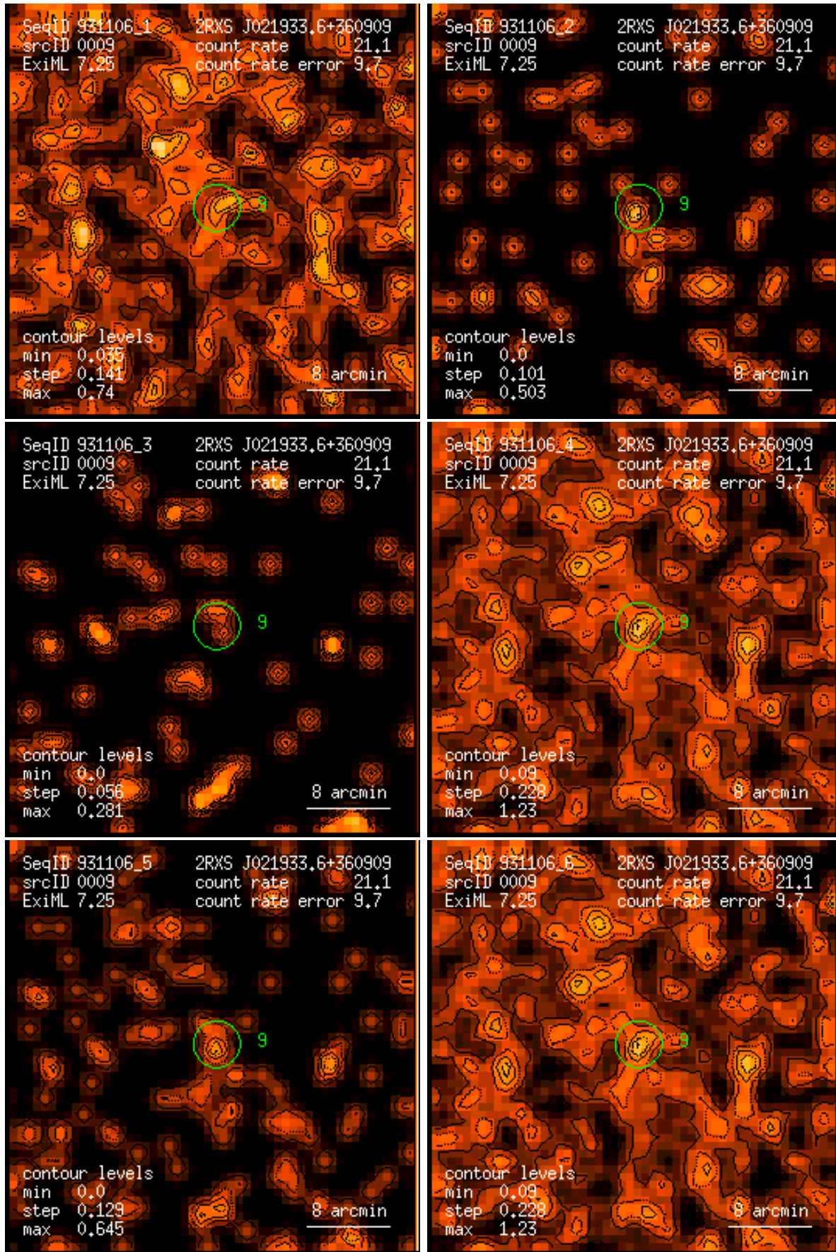
Figure 9: RASS 931106: detection 0009: band rate images, Gaussian filter: (1) PSPC channels 11 – 41, (2) 52 – 90, (3) 91 – 201, (4) 11 – 235, (5) 52 – 201, (6) 11 – 201. Broad band rates in counts/ks. Band rate contour levels in counts/ks/arcmin 2 .
