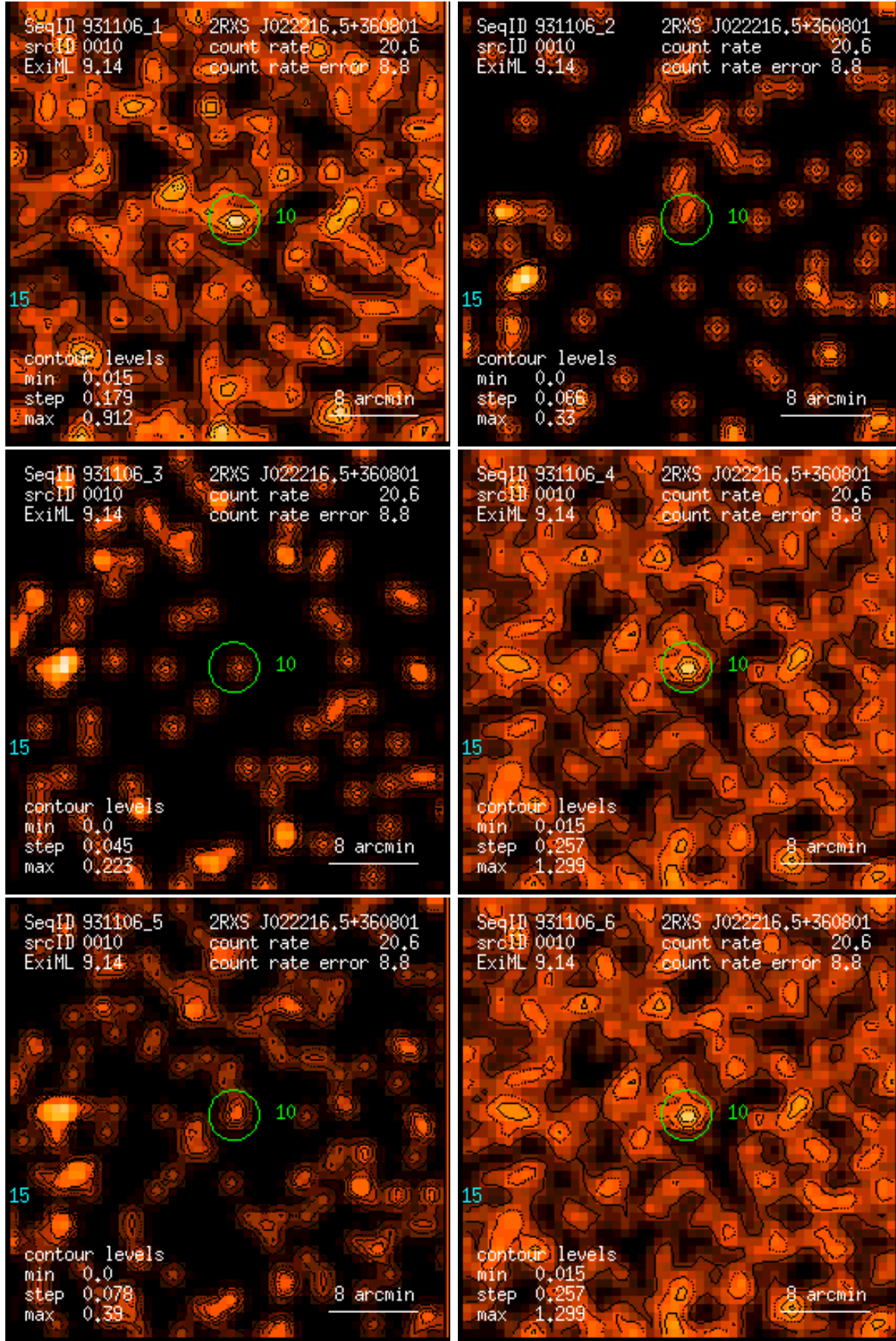
Figure 10: RASS 931106: detection 0010: band rate images, Gaussian filter: (1) PSPC channels 11 – 41, (2) 52 – 90, (3) 91 – 201, (4) 11 – 235, (5) 52 – 201, (6) 11 – 201. Broad band rates in counts/ks. Band rate contour levels in counts/ks/arcmin 2 .
