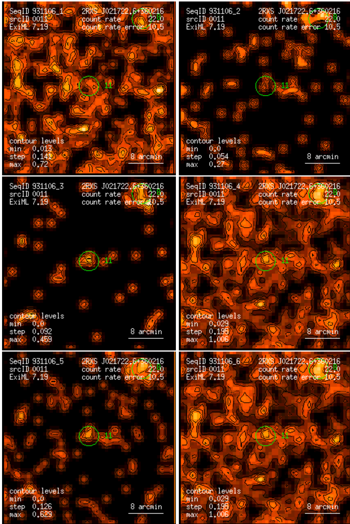
Figure 11: RASS 931106: detection 0011: band rate images, Gaussian filter: (1) PSPC channels 11 – 41, (2) 52 – 90, (3) 91 – 201, (4) 11 – 235, (5) 52 – 201, (6) 11 – 201. Broad band rates in counts/ks. Band rate contour levels in counts/ks/arcmin 2 .
