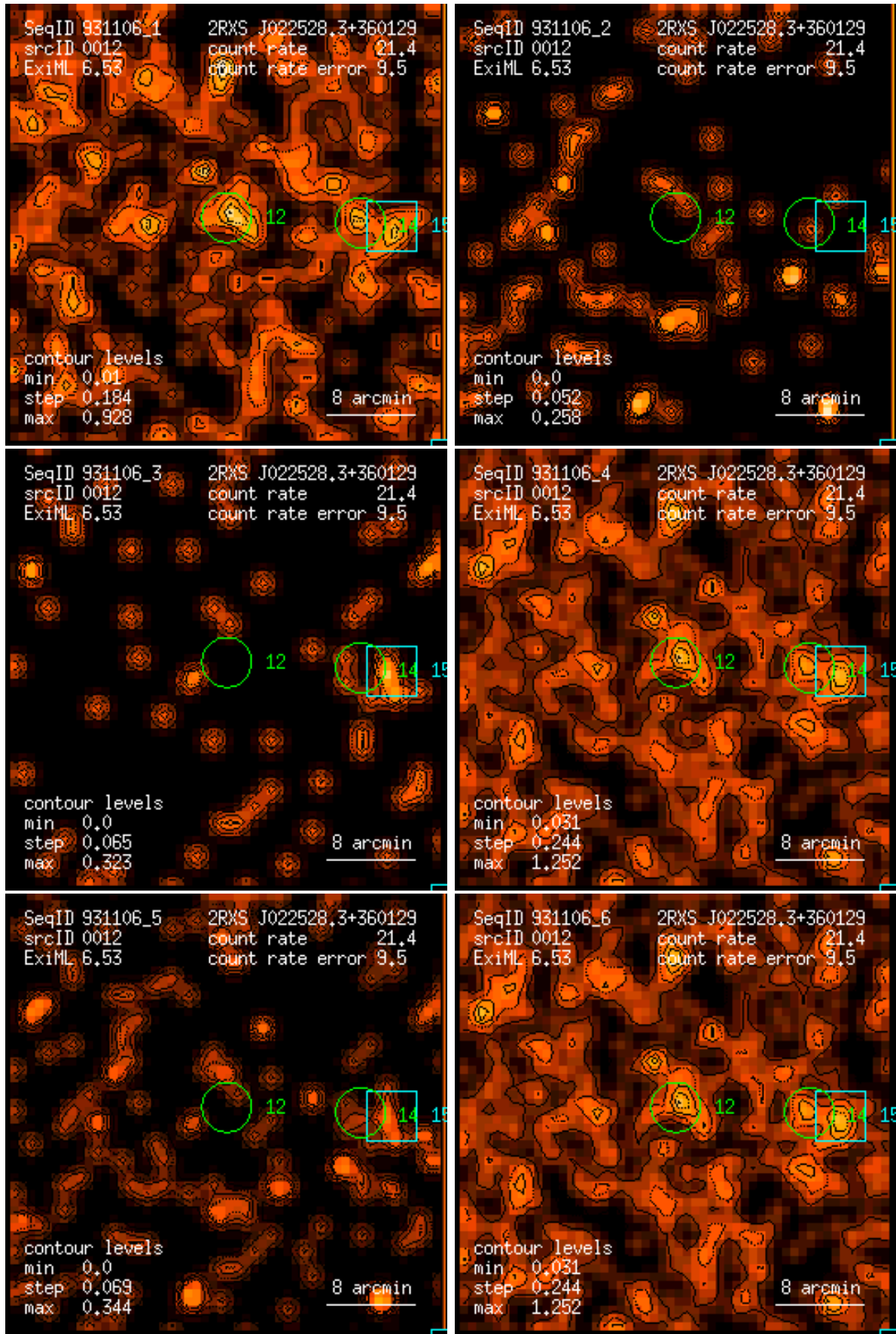
Figure 12: RASS 931106: detection 0012: band rate images, Gaussian filter: (1) PSPC channels 11 – 41, (2) 52 – 90, (3) 91 – 201, (4) 11 – 235, (5) 52 – 201, (6) 11 – 201. Broad band rates in counts/ks. Band rate contour levels in counts/ks/arcmin 2 .
