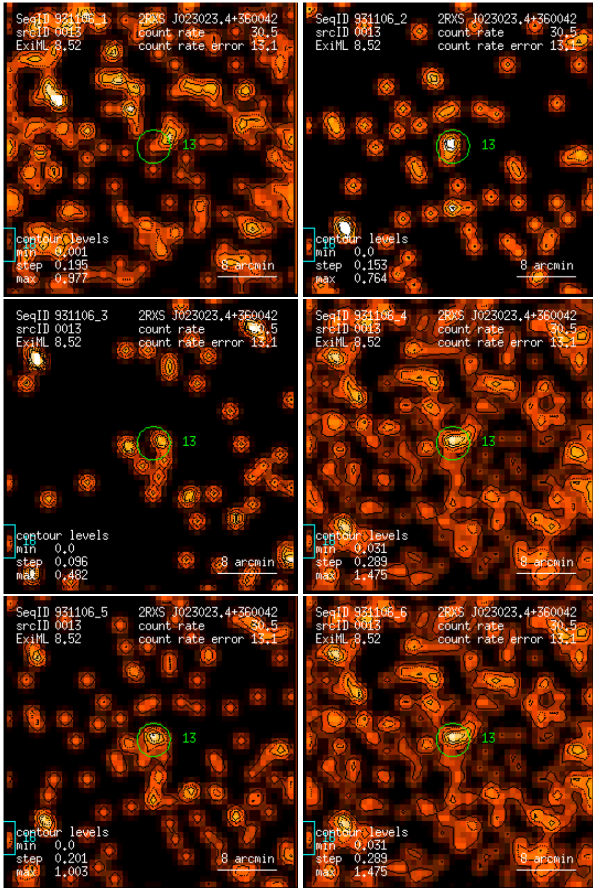
Figure 13: RASS 931106: detection 0013: band rate images, Gaussian filter: (1) PSPC channels 11 – 41, (2) 52 – 90, (3) 91 – 201, (4) 11 – 235, (5) 52 – 201, (6) 11 – 201. Broad band rates in counts/ks. Band rate contour levels in counts/ks/arcmin 2 .
