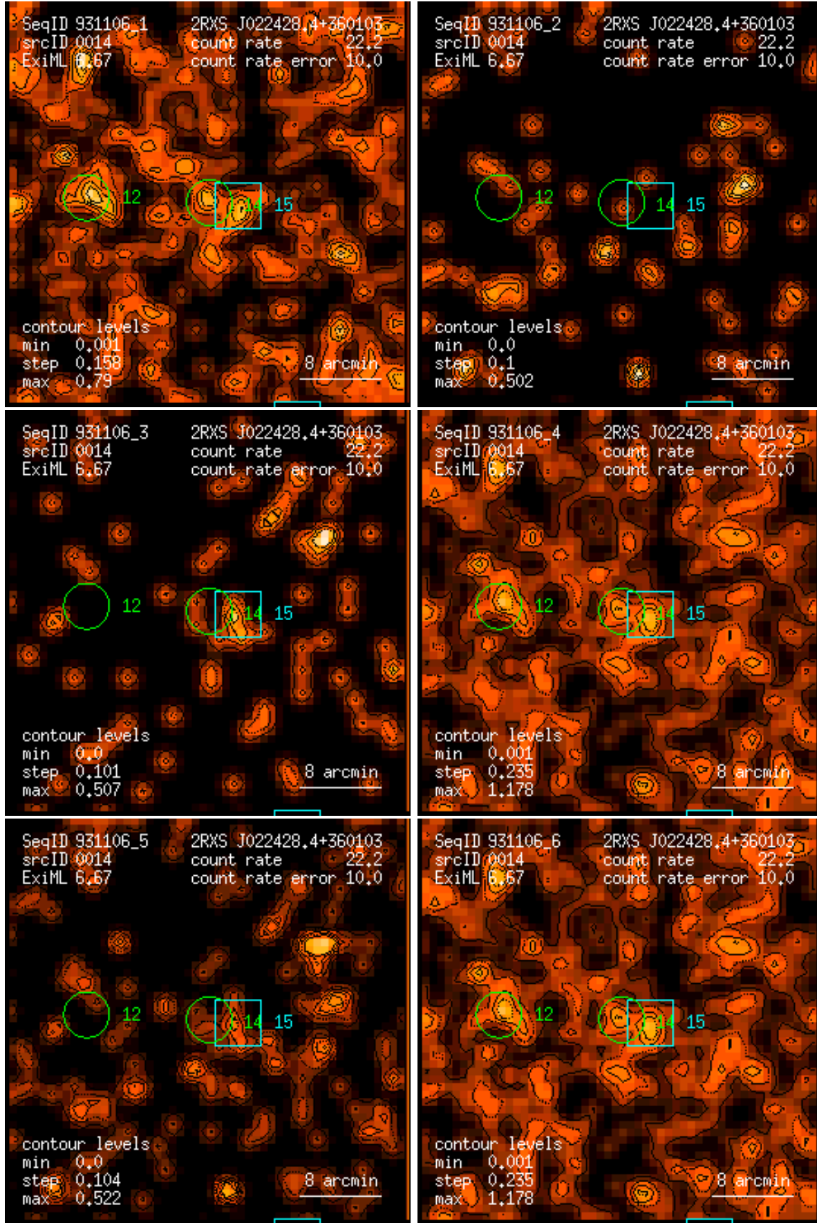
Figure 14: RASS 931106: detection 0014: band rate images, Gaussian filter: (1) PSPC channels 11 – 41, (2) 52 – 90, (3) 91 – 201, (4) 11 – 235, (5) 52 – 201, (6) 11 – 201. Broad band rates in counts/ks. Band rate contour levels in counts/ks/arcmin 2 .
