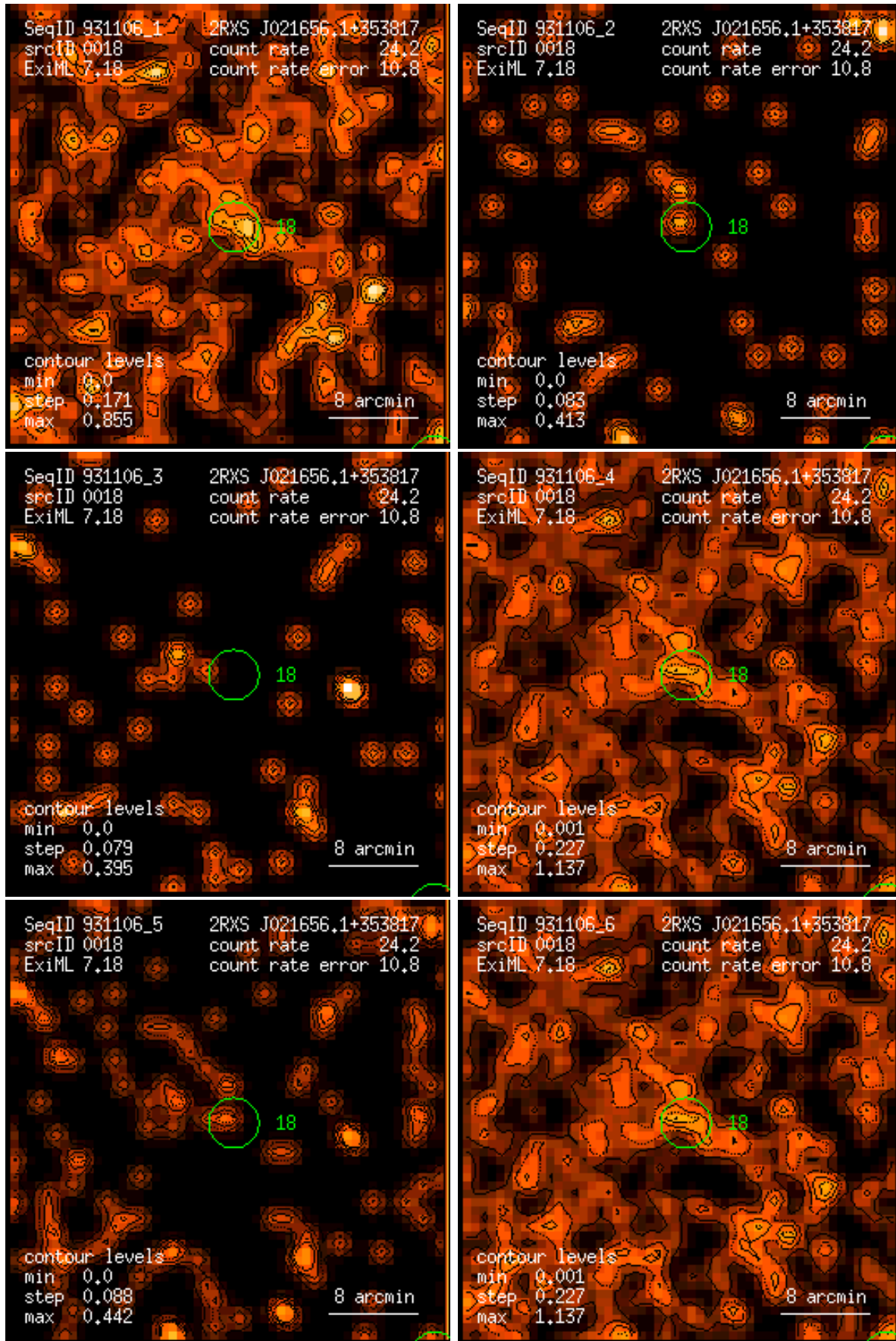
Figure 18: RASS 931106: detection 0018: band rate images, Gaussian filter: (1) PSPC channels 11 – 41, (2) 52 – 90, (3) 91 – 201, (4) 11 – 235, (5) 52 – 201, (6) 11 – 201. Broad band rates in counts/ks. Band rate contour levels in counts/ks/arcmin 2 .
