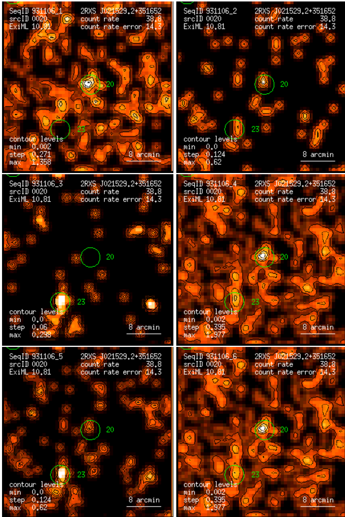
Figure 20: RASS 931106: detection 0020: band rate images, Gaussian filter: (1) PSPC channels 11 – 41, (2) 52 – 90, (3) 91 – 201, (4) 11 – 235, (5) 52 – 201, (6) 11 – 201. Broad band rates in counts/ks. Band rate contour levels in counts/ks/arcmin 2 .
