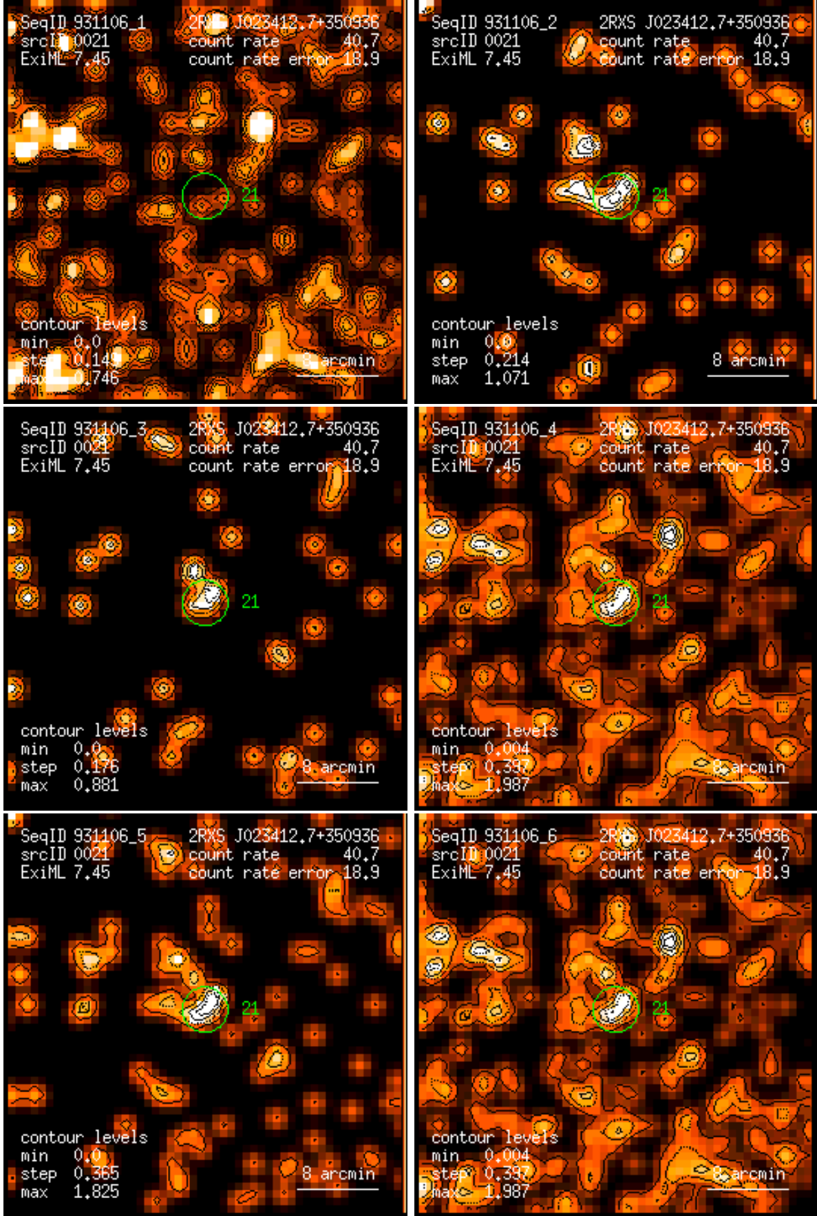
Figure 21: RASS 931106: detection 0021: band rate images, Gaussian filter: (1) PSPC channels 11 – 41, (2) 52 – 90, (3) 91 – 201, (4) 11 – 235, (5) 52 – 201, (6) 11 – 201. Broad band rates in counts/ks. Band rate contour levels in counts/ks/arcmin 2 .
