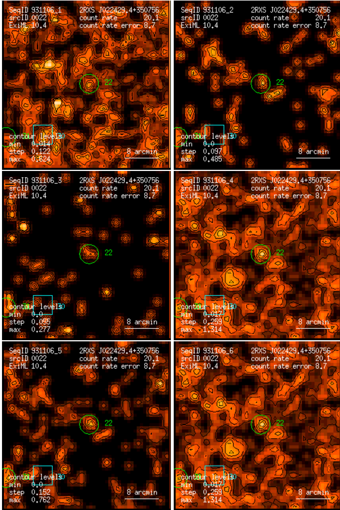
Figure 22: RASS 931106: detection 0022: band rate images, Gaussian filter: (1) PSPC channels 11 – 41, (2) 52 – 90, (3) 91 – 201, (4) 11 – 235, (5) 52 – 201, (6) 11 – 201. Broad band rates in counts/ks. Band rate contour levels in counts/ks/arcmin 2 .
