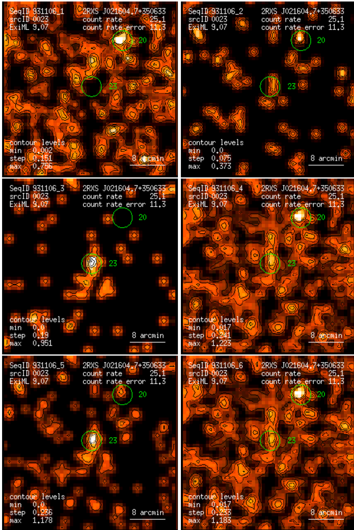
Figure 23: RASS 931106: detection 0023: band rate images, Gaussian filter: (1) PSPC channels 11 – 41, (2) 52 – 90, (3) 91 – 201, (4) 11 – 235, (5) 52 – 201, (6) 11 – 201. Broad band rates in counts/ks. Band rate contour levels in counts/ks/arcmin 2 .
