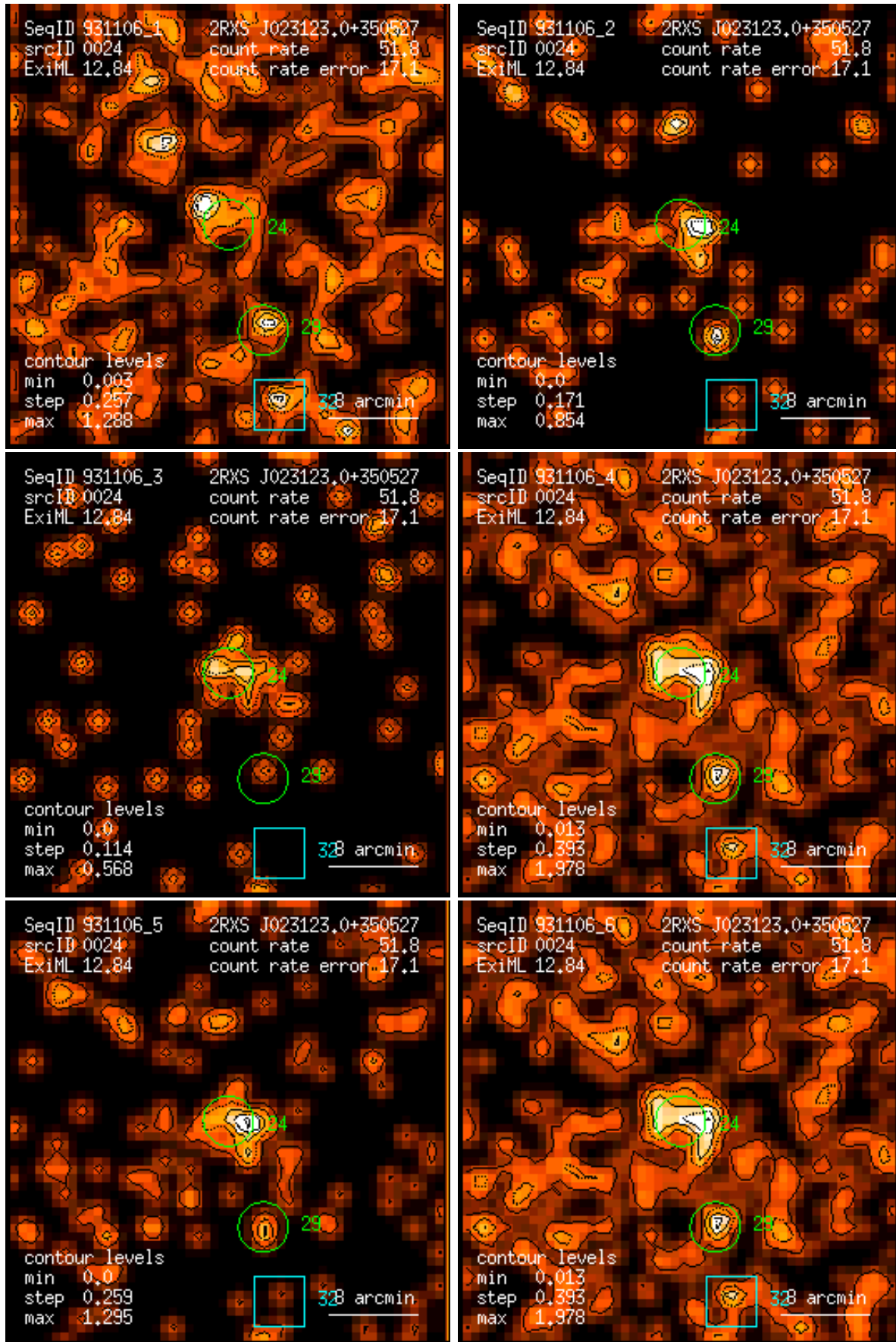
Figure 24: RASS 931106: detection 0024: band rate images, Gaussian filter: (1) PSPC channels 11 – 41, (2) 52 – 90, (3) 91 – 201, (4) 11 – 235, (5) 52 – 201, (6) 11 – 201. Broad band rates in counts/ks. Band rate contour levels in counts/ks/arcmin 2 .
