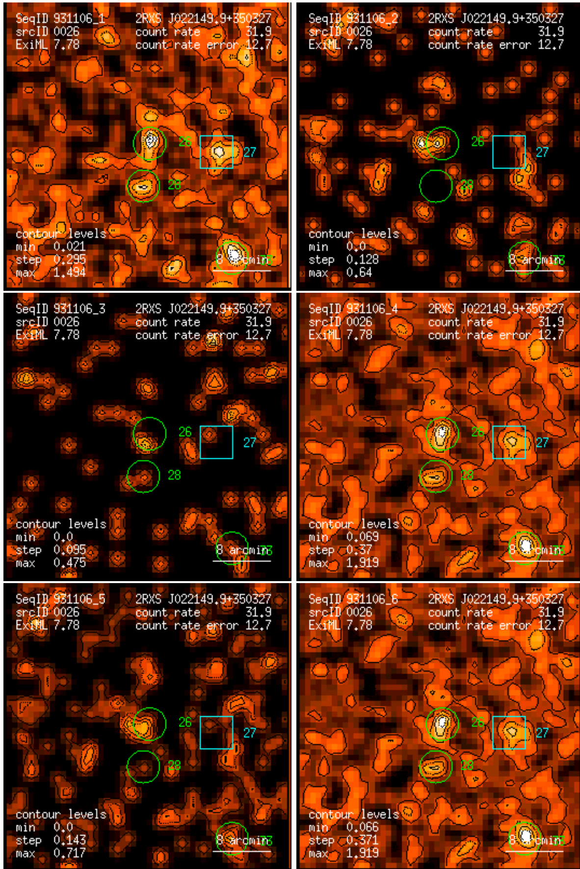
Figure 26: RASS 931106: detection 0026: band rate images, Gaussian filter: (1) PSPC channels 11 – 41, (2) 52 – 90, (3) 91 – 201, (4) 11 – 235, (5) 52 – 201, (6) 11 – 201. Broad band rates in counts/ks. Band rate contour levels in counts/ks/arcmin 2 .
