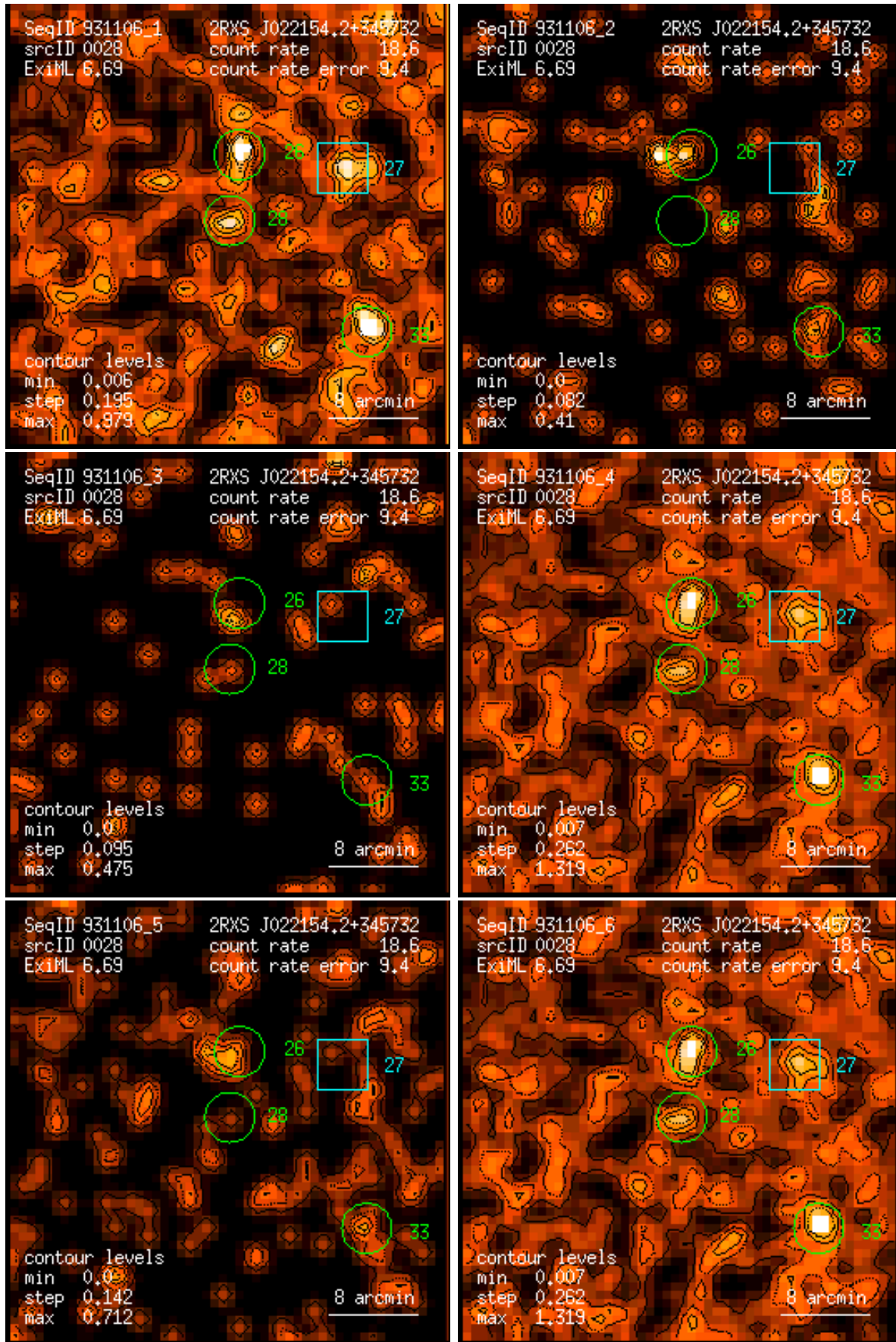
Figure 28: RASS 931106: detection 0028: band rate images, Gaussian filter: (1) PSPC channels 11 – 41, (2) 52 – 90, (3) 91 – 201, (4) 11 – 235, (5) 52 – 201, (6) 11 – 201. Broad band rates in counts/ks. Band rate contour levels in counts/ks/arcmin 2 .
