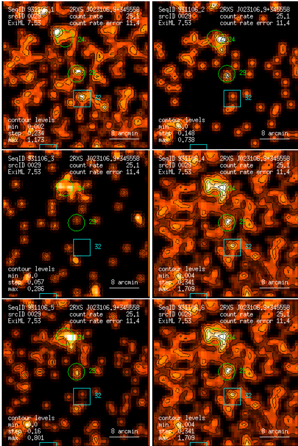
Figure 29: RASS 931106: detection 0029: band rate images, Gaussian filter: (1) PSPC channels 11 – 41, (2) 52 – 90, (3) 91 – 201, (4) 11 – 235, (5) 52 – 201, (6) 11 – 201. Broad band rates in counts/ks. Band rate contour levels in counts/ks/arcmin 2 .
