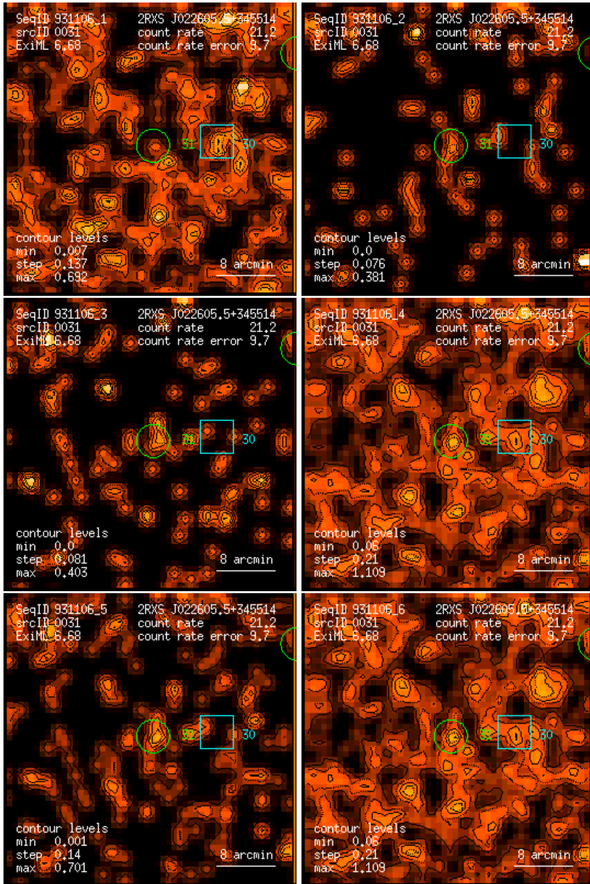
Figure 31: RASS 931106: detection 0031: band rate images, Gaussian filter: (1) PSPC channels 11 – 41, (2) 52 – 90, (3) 91 – 201, (4) 11 – 235, (5) 52 – 201, (6) 11 – 201. Broad band rates in counts/ks. Band rate contour levels in counts/ks/arcmin 2 .
