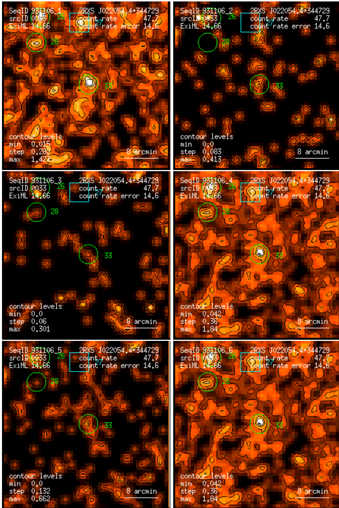
Figure 33: RASS 931106: detection 0033: band rate images, Gaussian filter: (1) PSPC channels 11 – 41, (2) 52 – 90, (3) 91 – 201, (4) 11 – 235, (5) 52 – 201, (6) 11 – 201. Broad band rates in counts/ks. Band rate contour levels in counts/ks/arcmin 2 .
