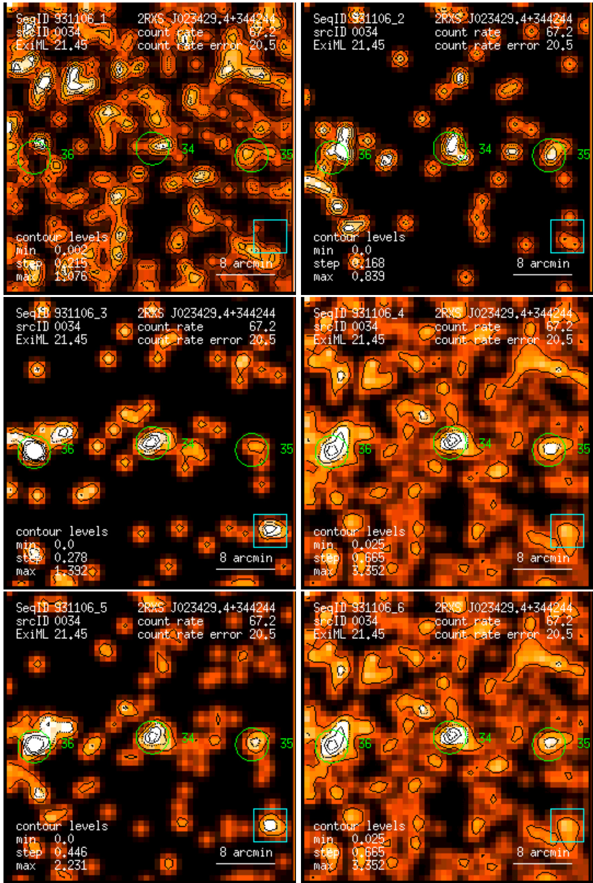
Figure 34: RASS 931106: detection 0034: band rate images, Gaussian filter: (1) PSPC channels 11 – 41, (2) 52 – 90, (3) 91 – 201, (4) 11 – 235, (5) 52 – 201, (6) 11 – 201. Broad band rates in counts/ks. Band rate contour levels in counts/ks/arcmin 2 .
