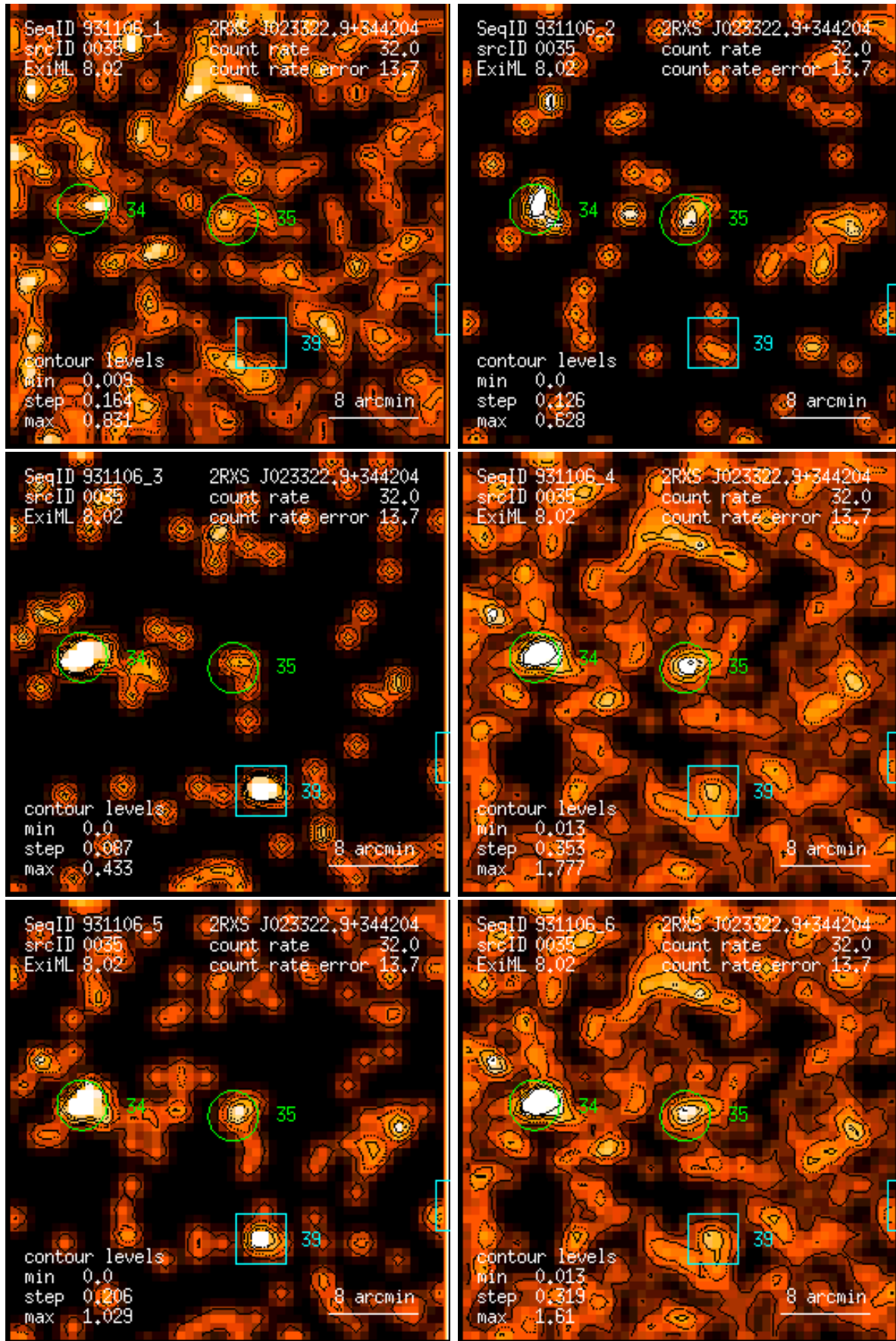
Figure 35: RASS 931106: detection 0035: band rate images, Gaussian filter: (1) PSPC channels 11 – 41, (2) 52 – 90, (3) 91 – 201, (4) 11 – 235, (5) 52 – 201, (6) 11 – 201. Broad band rates in counts/ks. Band rate contour levels in counts/ks/arcmin 2 .
