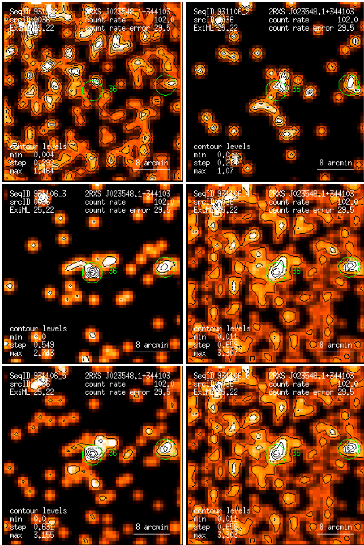
Figure 36: RASS 931106: detection 0036: band rate images, Gaussian filter: (1) PSPC channels 11 – 41, (2) 52 – 90, (3) 91 – 201, (4) 11 – 235, (5) 52 – 201, (6) 11 – 201. Broad band rates in counts/ks. Band rate contour levels in counts/ks/arcmin 2 .
