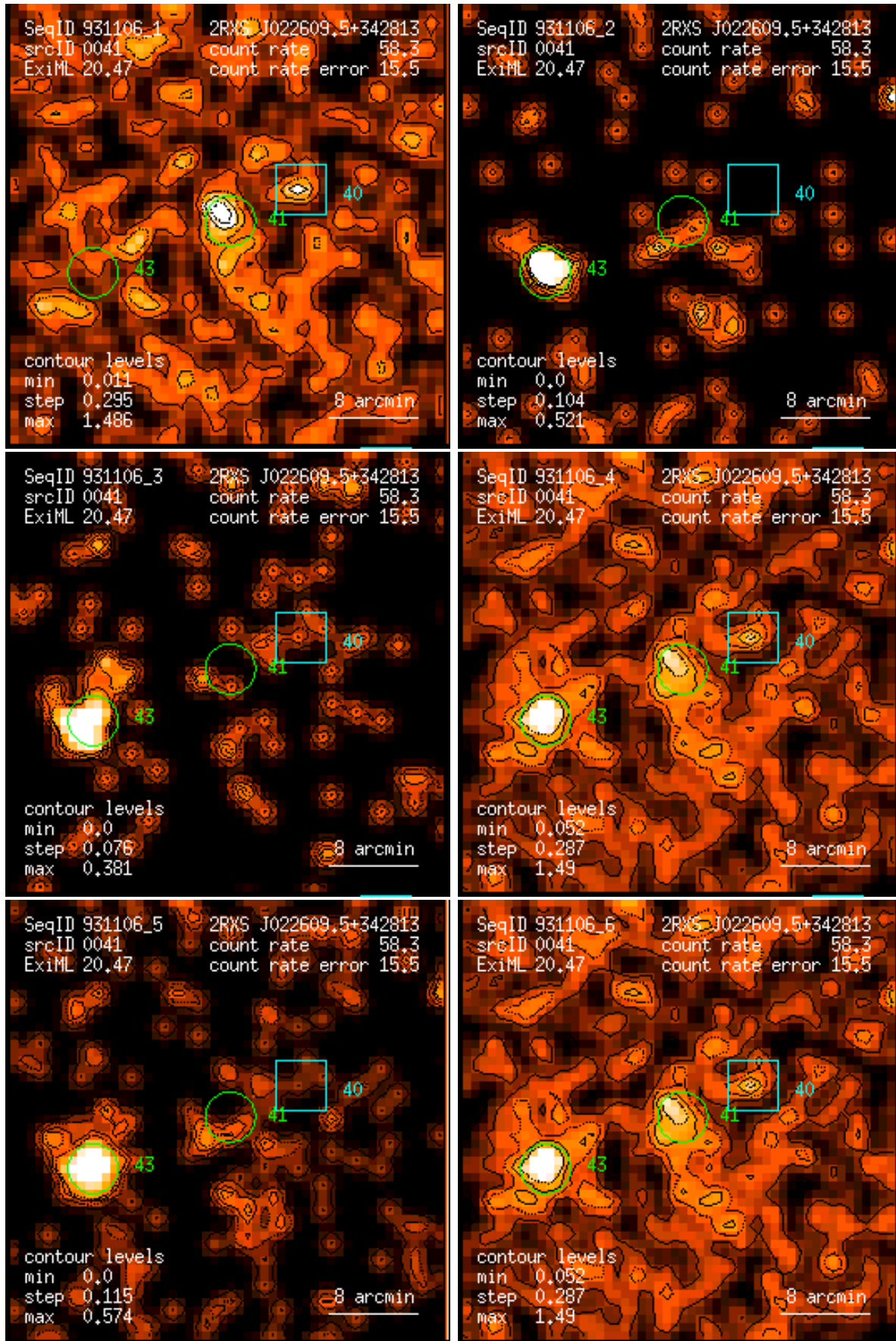
Figure 41: RASS 931106: detection 0041: band rate images, Gaussian filter: (1) PSPC channels 11 – 41, (2) 52 – 90, (3) 91 – 201, (4) 11 – 235, (5) 52 – 201, (6) 11 – 201. Broad band rates in counts/ks. Band rate contour levels in counts/ks/arcmin 2 .
