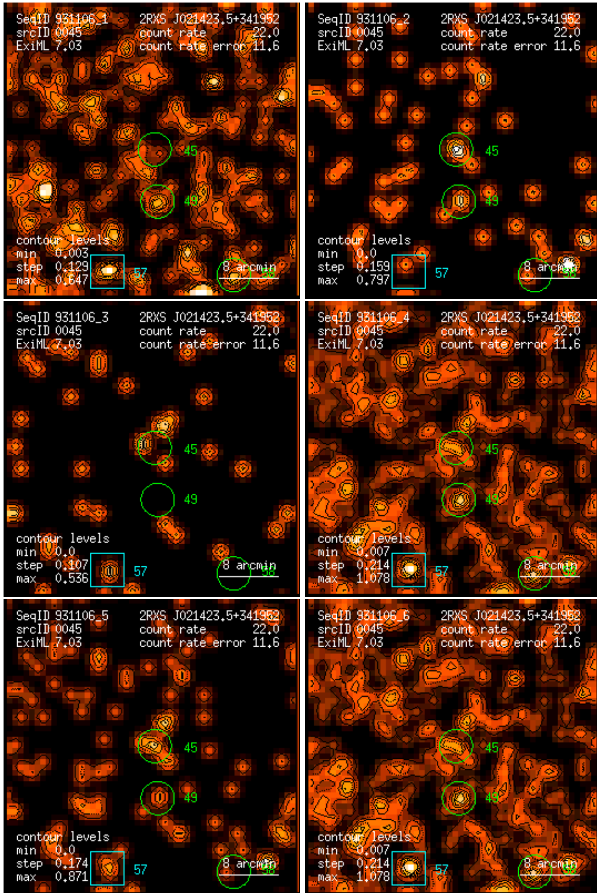
Figure 45: RASS 931106: detection 0045: band rate images, Gaussian filter: (1) PSPC channels 11 – 41, (2) 52 – 90, (3) 91 – 201, (4) 11 – 235, (5) 52 – 201, (6) 11 – 201. Broad band rates in counts/ks. Band rate contour levels in counts/ks/arcmin 2 .
