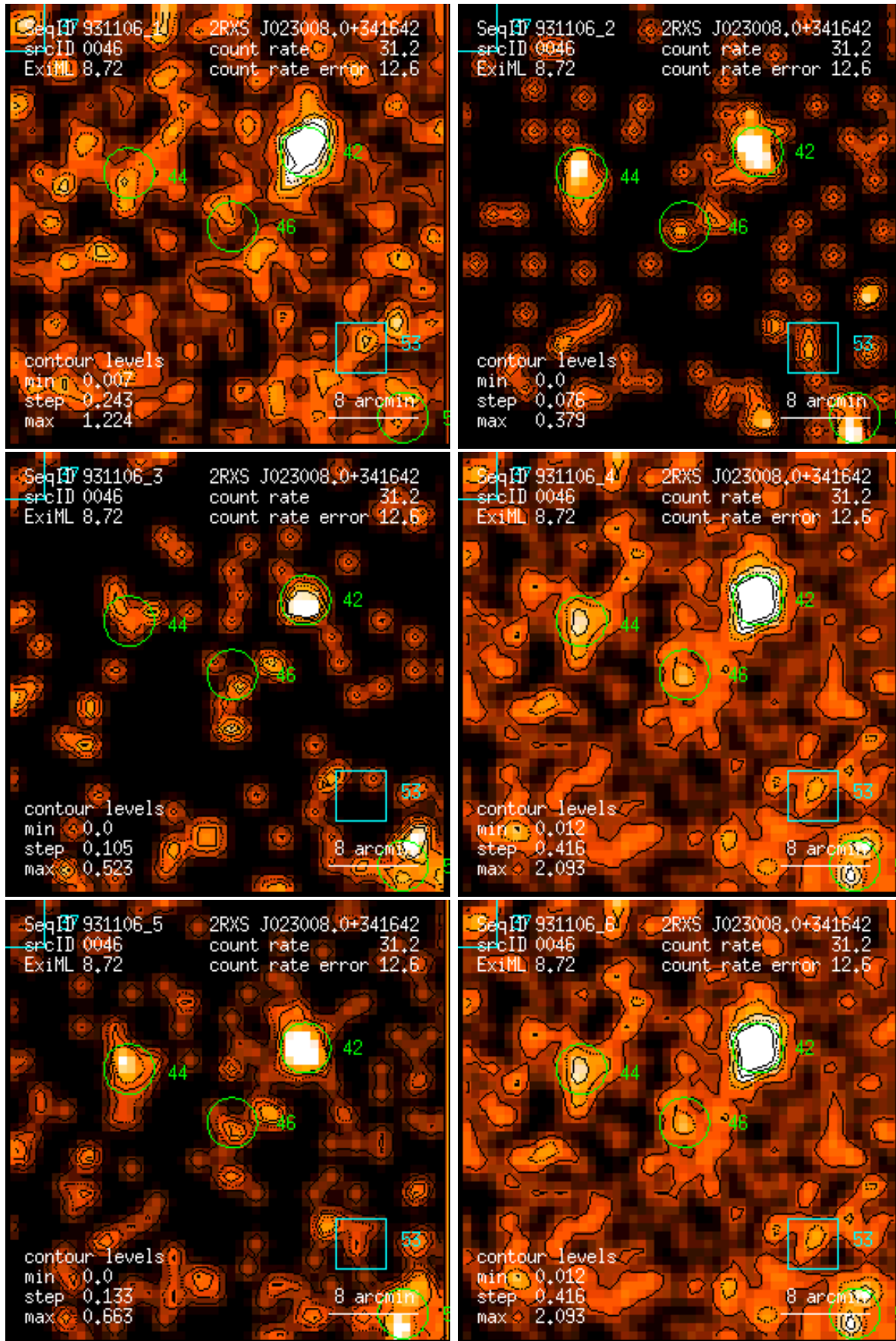
Figure 46: RASS 931106: detection 0046: band rate images, Gaussian filter: (1) PSPC channels 11 – 41, (2) 52 – 90, (3) 91 – 201, (4) 11 – 235, (5) 52 – 201, (6) 11 – 201. Broad band rates in counts/ks. Band rate contour levels in counts/ks/arcmin 2 .
