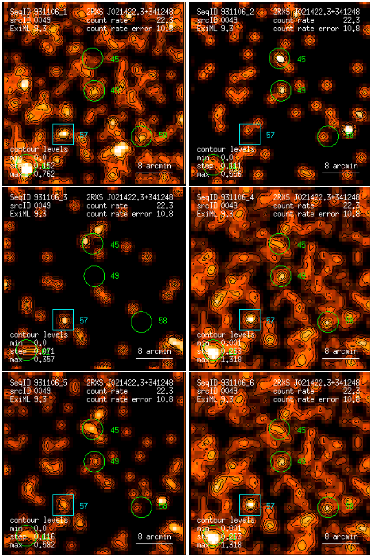
Figure 49: RASS 931106: detection 0049: band rate images, Gaussian filter: (1) PSPC channels 11 – 41, (2) 52 – 90, (3) 91 – 201, (4) 11 – 235, (5) 52 – 201, (6) 11 – 201. Broad band rates in counts/ks. Band rate contour levels in counts/ks/arcmin 2 .
