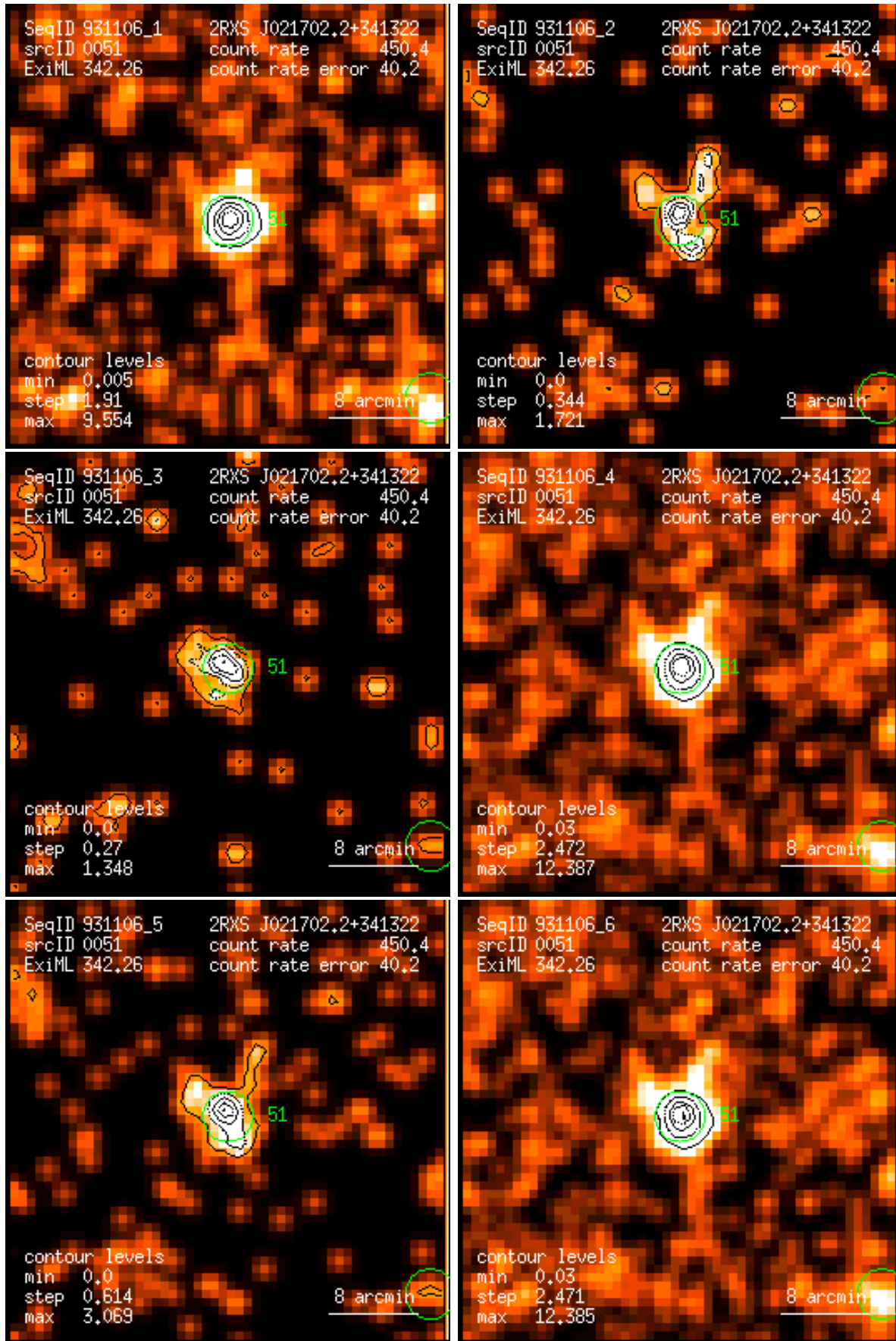
Figure 51: RASS 931106: detection 0051: band rate images, Gaussian filter: (1) PSPC channels 11 – 41, (2) 52 – 90, (3) 91 – 201, (4) 11 – 235, (5) 52 – 201, (6) 11 – 201. Broad band rates in counts/ks. Band rate contour levels in counts/ks/arcmin 2 .
