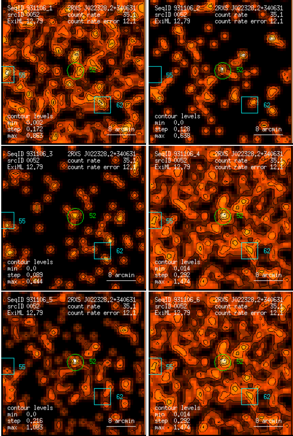
Figure 52: RASS 931106: detection 0052: band rate images, Gaussian filter: (1) PSPC channels 11 – 41, (2) 52 – 90, (3) 91 – 201, (4) 11 – 235, (5) 52 – 201, (6) 11 – 201. Broad band rates in counts/ks. Band rate contour levels in counts/ks/arcmin 2 .
